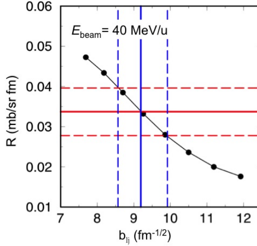
Fig. 1. (Color online) Expected dependency (black points) of the ratio R = \sigma^{\text{DW}}/b_{\ell j}^2 (units of mb/sr-fm) at \approx 40 MeV/u as a function of the single-particle ANC b_{\ell j} in units of \text{fm}^{-1/2} . The solid/red horizontal line is the centroid of the R value determined from the peripheral reaction with uncertainties given by the dashed/red lines. The solid/blue vertical line is the central value for the b_{\ell j} constrained by the R measured at \approx 5 MeV/u, with the dashed/blue lines giving the uncertainties in determining b_{\ell j} .
