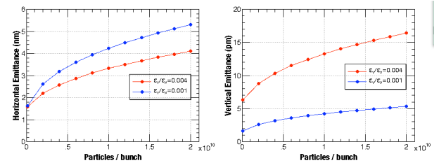
Figure 2: Horizontal (left) and vertical (right) equilibrium emittances vs. particles/bunch with intrabeam scattering, for two emittance ratios.
