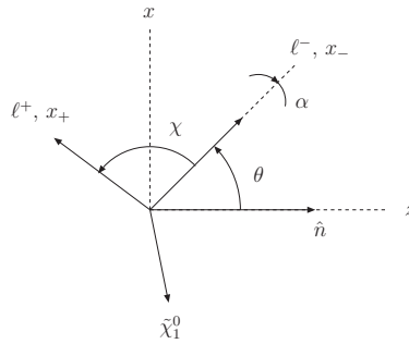
Fig. 1. Kinematic configuration of momenta and the spin vector in the neutralino \tilde{\chi}_2^0 rest frame.
