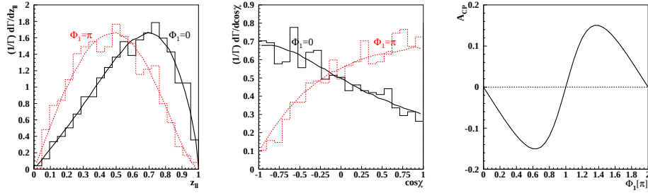
Fig. 3. The lepton invariant mass distribution (the left panel) and the opening angle distribution (the middle panel). The solid (dashed) lines are for \Phi_1 = 0 ( \Phi_1 = \pi ), i.e. for neutralinos with the same (opposite) CP parities. The right panel: the \Phi_1 dependence of the A_{\text{CP}} (11).
