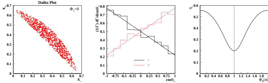
Fig. 2. Left: the Dalitz plot for the neutralino \tilde{\chi}_2^0 decay. Middle: the normalized lepton angle distribution (8); the solid (dashed) line is for \ell^- ( \ell^+ ). Right: the \Phi_1 dependence of the slope parameter \eta_- for the parameter set (6).
