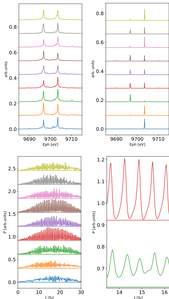
Figure 4: Measured FEL spectra (top left subplot with filtered subset representing best 1% of events in terms of peaks ratio and pulse energy) and simulated spectra (top right plot) with corresponding power profiles (bottom left plot). The bottom right plot depicts an enlarged part of the left plot, illustrating events with good and poor contrast.
