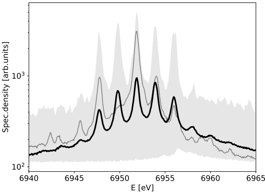
Figure 2: Radiation power spectrum as a function of photon energy for the case of seeding with 5 equidistant reflections. Also we can already see non-linear effects as additional maxima on both sides. Black line depicts the ensemble average over the ensemble of 10000 events, dark grey line shows a single-shot spectrum, light grey band represents the range of maximum and minimum values in the ensemble.
