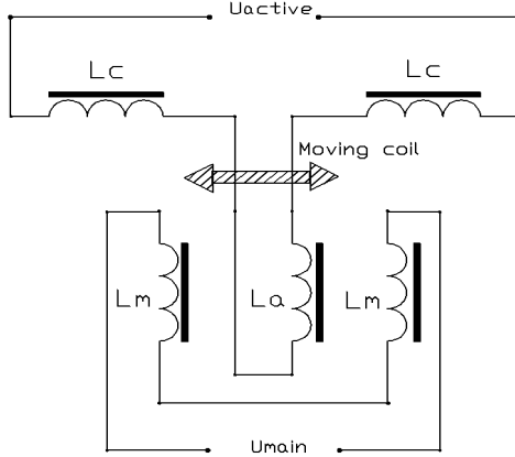
Figure 2: Tuner scheme.
