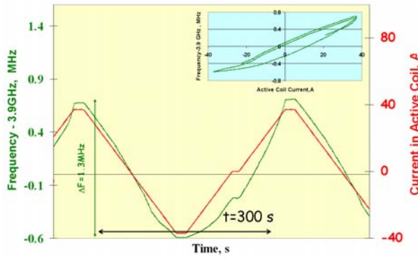
Figure 5: Cavity slow tuning ( I_m = 30 A, I_a = \pm 37 A) .
