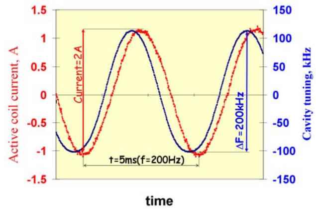
Figure 7: Tuner fast mode of operation. The active coil current is ( f = 200 Hz and I_a = 2 A), I_m = 30 A .
