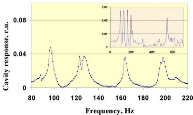
Figure 6: Cavity-tuner system transfer function. Active coil excited with sine wave current drive signal. Frequency of drive signal swept from 20 Hz up to 700 Hz.
