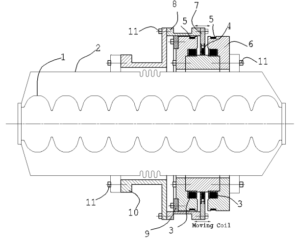
Figure 1: Electromagnetic Tuner cross-section.
