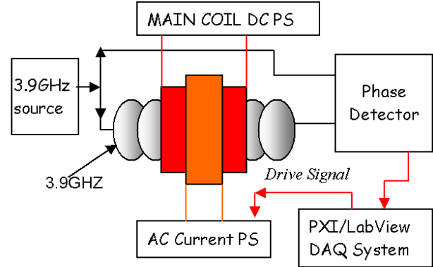
Figure 4: Phase detection scheme.
