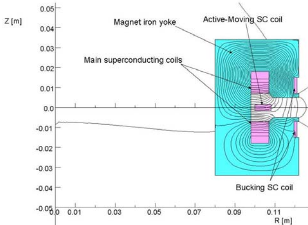
Figure 3: Magnet cross-section and flux lines.
