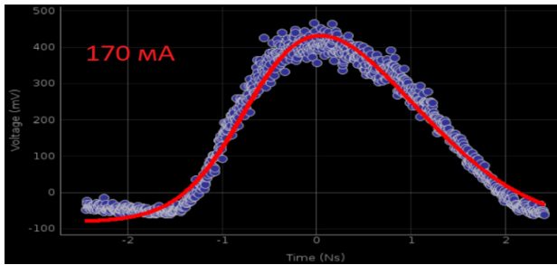
Figure 9: Longitudinal beam distribution (170 mA current) fitted by model (3).
