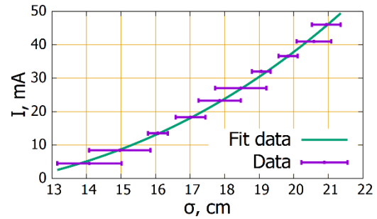
Figure 5: Longitudinal beam size vs. beam current (streak-camera).
