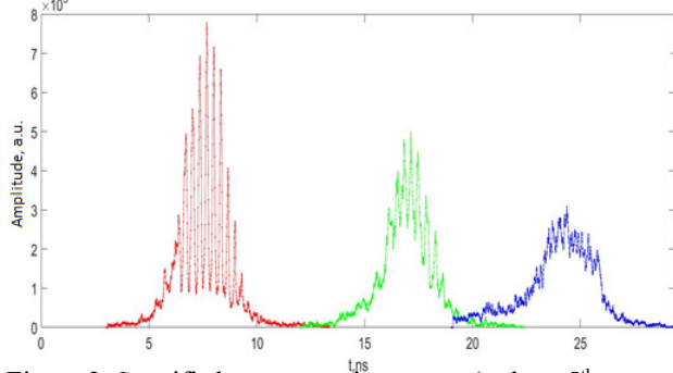
Figure 3: Specific beam grouping stages (red – 5 th turn, green – 25 th , blue – 115 th ).
