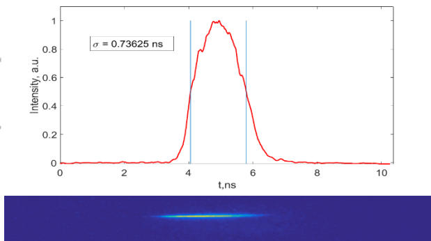
Figure 4: Beam particle distribution and beam profile (27 mA current, about 22 cm length).
