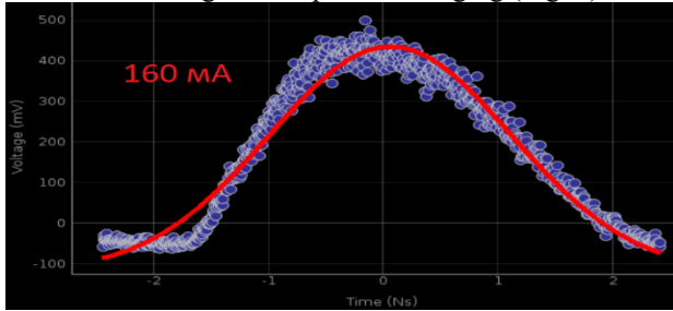
Figure 8: Longitudinal beam distribution (160 mA current) fitted by Gauss.
