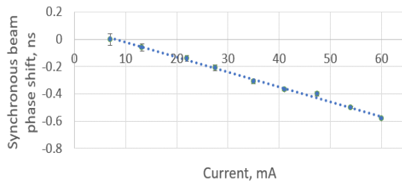
Figure 10. Synchronous beam phase shift vs. current.
