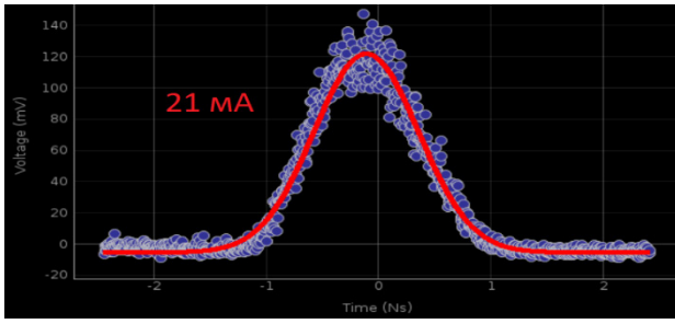
Figure 7: Longitudinal beam distribution (21 mA current) fitted by Gauss.
