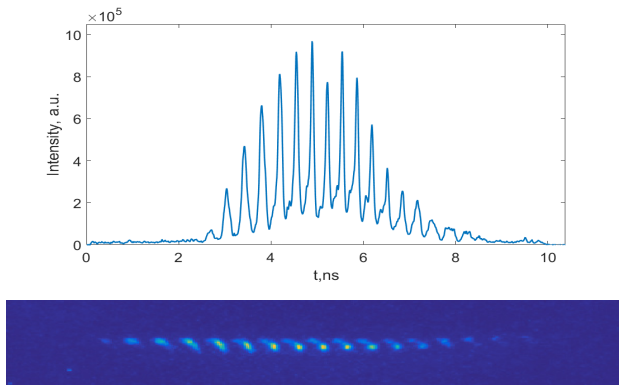
Figure 2: 16 bunches from linear accelerator.
