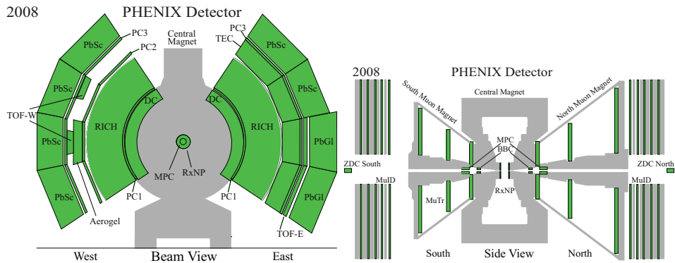
Fig. 1. PHENIX detector setup: (left) Central Arms in beam view; (right) Muon Arms in side view.
