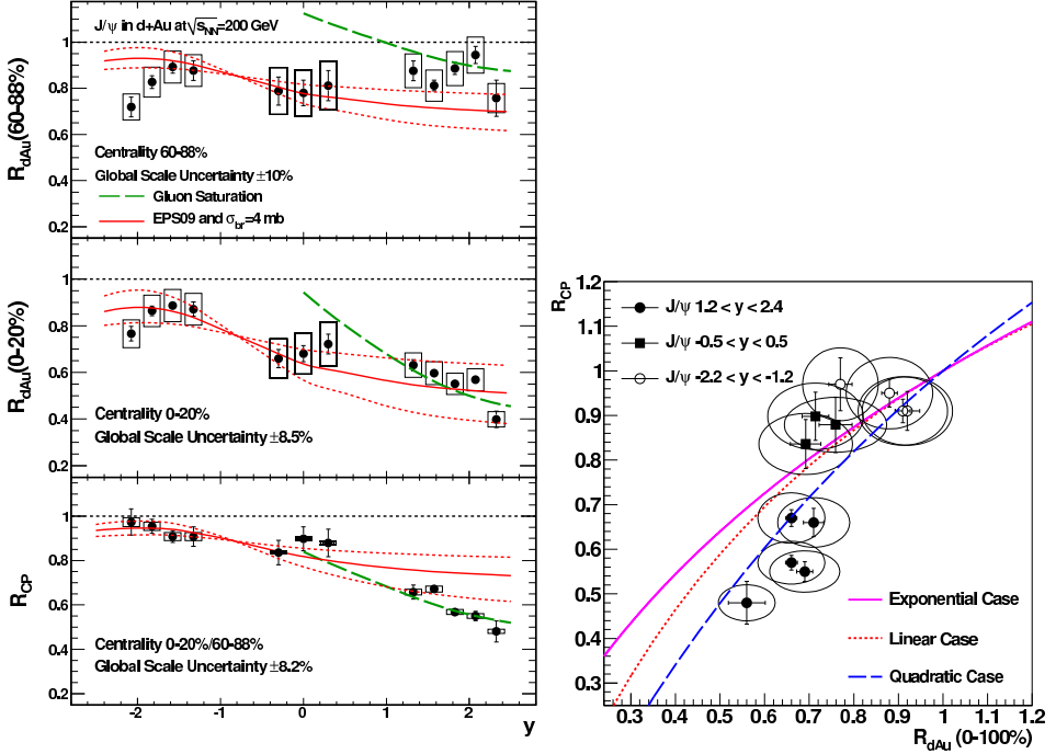
Fig. 5. (Left) Rapidity dependence of nuclear modification factors. (Right) Unbiased R_{dAu} vs. R_{CP} with different geometric dependencies of the nuclear modification.
