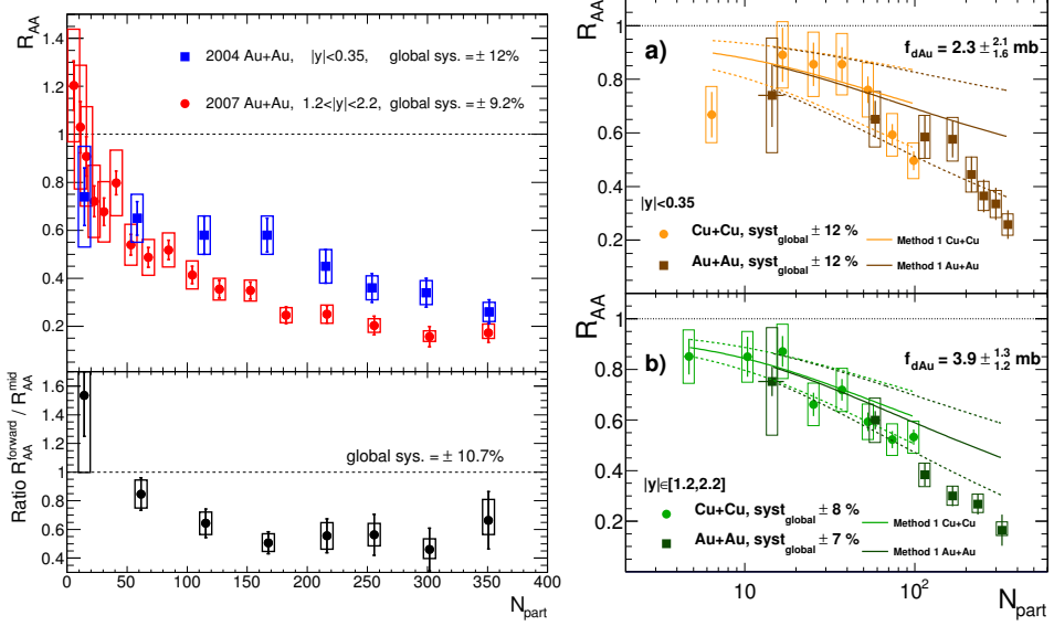
Fig. 2. (Color online) J/\psi R_{AA} as a function of the number of participants in Au+Au (left) and Cu+Cu (right) collisions at \sqrt{s_{NN}} = 200 GeV.
