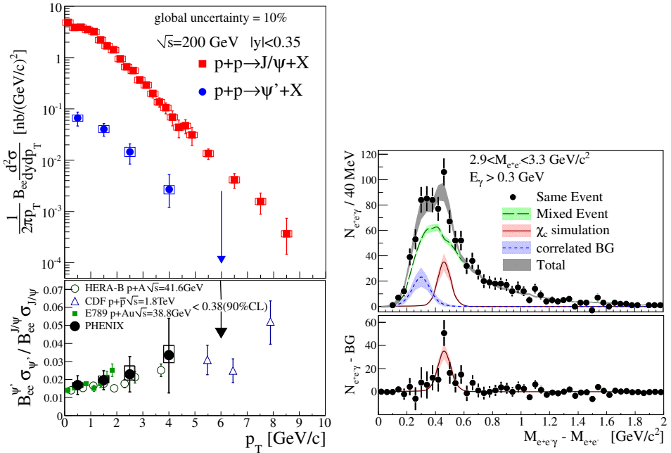
Fig. 4. (Color online) (left) Transverse momentum dependence of J/\psi and \psi' in |y| < 0.35 and their ratio at the bottom panel. (Right) e^+e^-\gamma invariant mass distribution and bottom panel is the \chi_c signal after like-sign background subtraction.
