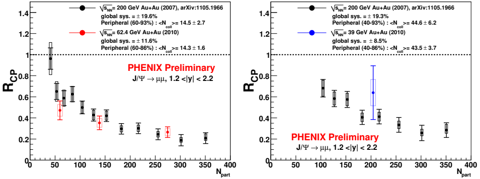
Fig. 3. J/\psi R_{CP} at \sqrt{s_{NN}} = 62 GeV (left) and 39 GeV (right) compared to the corresponding \sqrt{s_{NN}} = 200 GeV using the same peripheral bin as reference.
