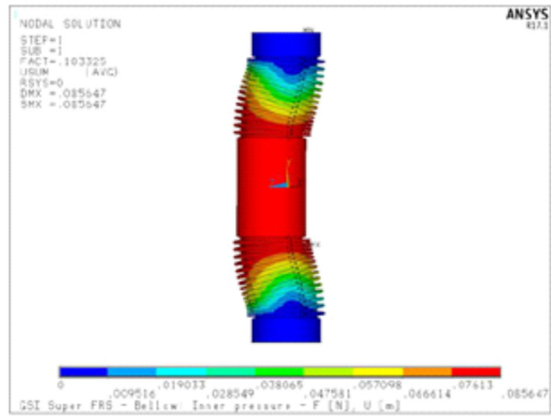
Figure 4: Deformation of the (lower) bellow containing the safety valve duct (in a circle) is clearly visible. This was observed after a pressure test at 8.3 bars. The viewports on the vacuum vessel are installed to measure cold mass movement during cool down (left). The FEM analysis result of the bellow buckling (right).
