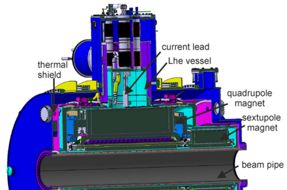
Figure 1: Cross section of the FoS Multiplet.
