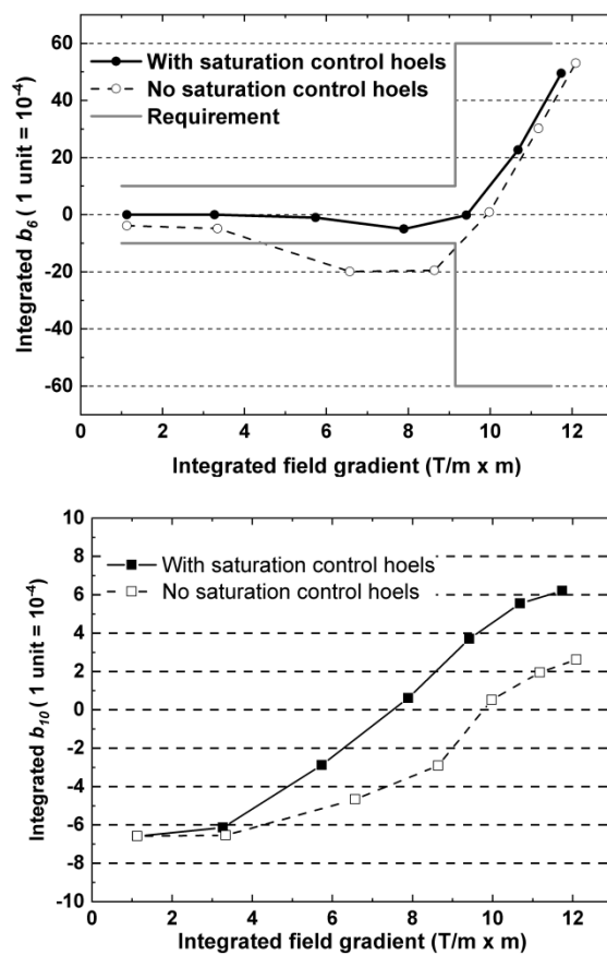
Figure 2: b_6 as a function of integrated gradient (top). The solid lines indicate the field quality requirement. b_{10} as a function of integrated gradient (bottom).
