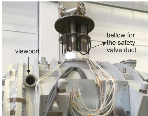
Figure 4: Deformation of the (lower) bellow containing the safety valve duct (in a circle) is clearly visible. This was observed after a pressure test at 8.3 bars. The viewports on the vacuum vessel are installed to measure cold mass movement during cool down (left). The FEM analysis result of the bellow buckling (right).
