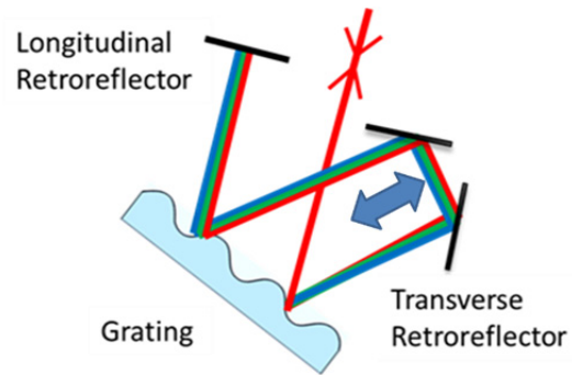
Figure 4: Schematic of the pulse stretcher system.
