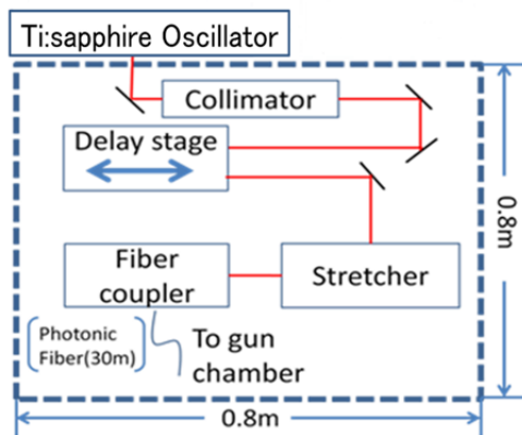
Figure 3: Schematic of the laser system.
