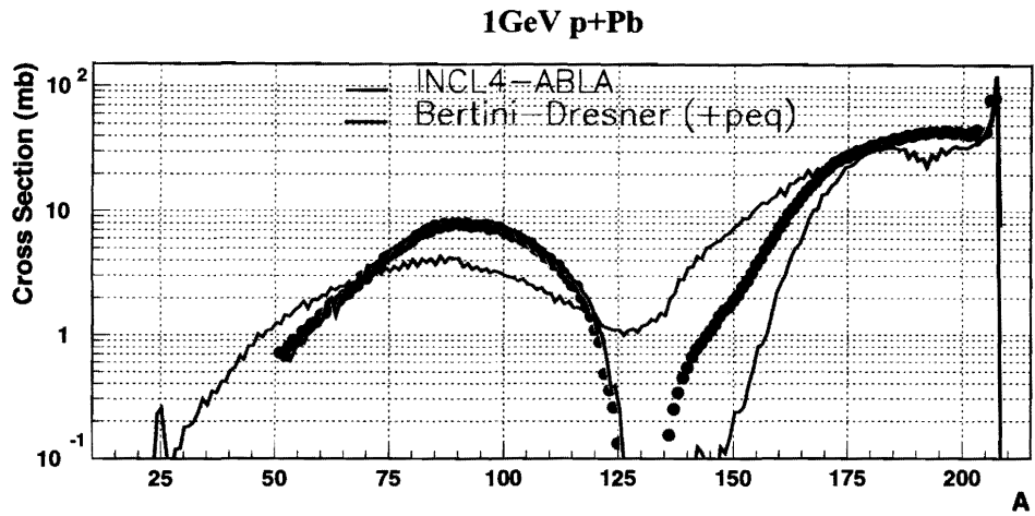
Fig.1. Comparison of INCL4-ABLA 5,6) and Bertini-Dresner 9,10) predictions with the production cross-sections (mb) as a function of the residue masses measured at GSI with the reverse kinematics technique in for the p+Pb system 2) .
