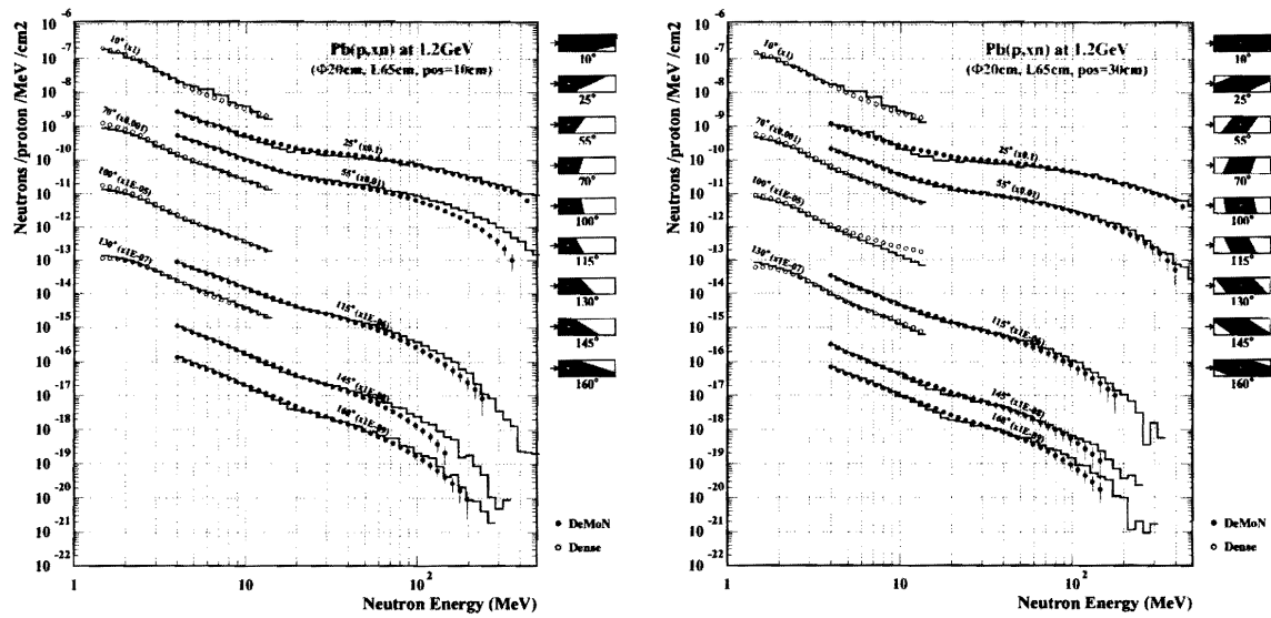
Fig. 4: Neutron spectra (number of neutrons per incident proton, MeV and cm 2 of detector) measured at SATURNE 4) on a 20 cm diameter lead target at 1.2 GeV (black points) compared with calculations 146) made with the LAHET3/MCNP code using the INCL4/ABLA model combination (red line). The two figures correspond to two different longitudinal positions of the target with respect to the collimators. On each figure and for each angle a diagram showing the full exposition and penumbra zone due to the presence of the collimators has been added.
