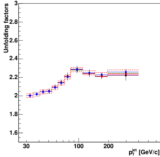
Figure 4.14: Unfolding factors for the p_T^{\text{jet}} distribution in Z/\gamma^*(\rightarrow e^+e^-) + \geq 1 jet events. Black dots represent the unfolding factors using non-reweighted PYTHIA-TUNE A, red dots for PYTHIA-TUNE A reweighted only on \hat{p}_T , green and pink dots varying up and down the weighting function, and blue dots for the unfolding factors reweighted on both \hat{p}_T and E_T^{e, \text{fwd}} . The dashed lines correspond to the assigned uncertainty of 1%.
