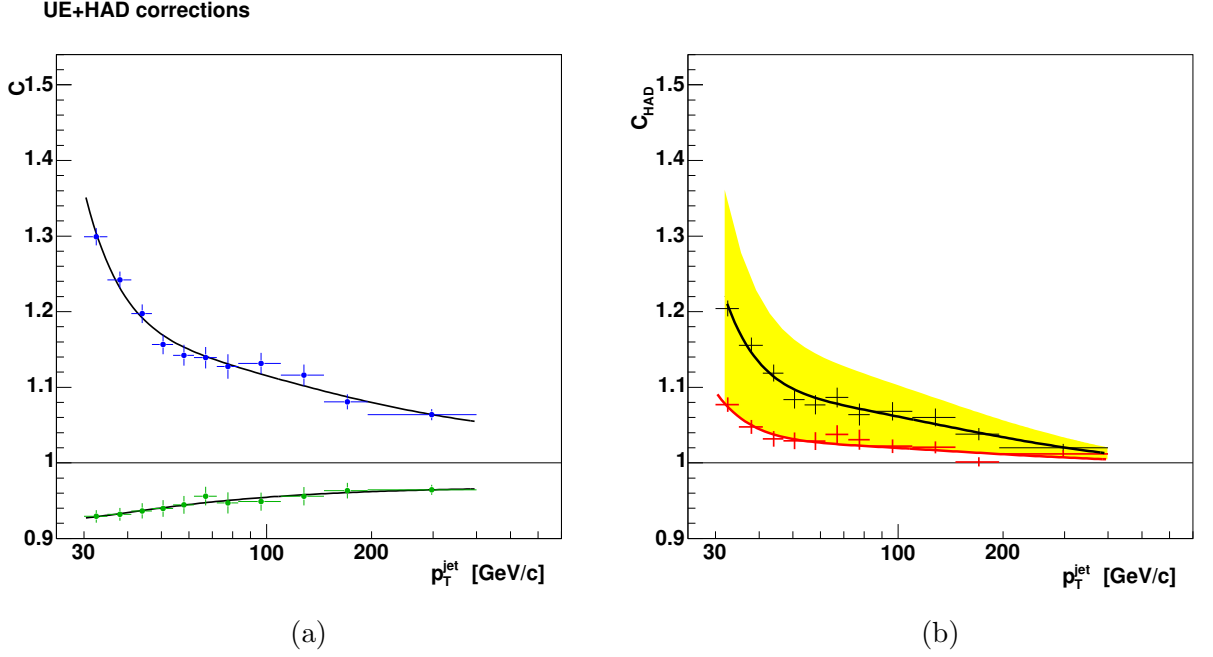
Figure 6.1: (a) C_{\text{UE}} (blue) and C_{\text{hadronization}} (green) corrections for Z/\gamma^*(\rightarrow e^+e^-) + \geq 1 jet cross section. (b) Global C_{\text{HAD}} correction factors determined using PYTHIA TUNE A (black) and using TUNE DW (red). The nominal correction is TUNE A and the yellow band indicates the assigned systematic uncertainty that is the symmetrized difference between TUNE A and TUNE DW corrections.
