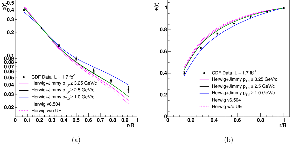
Figure 5.6: (a) Differential and (b) integrated jet shapes for jets with p_T^{\text{jet}} > 30 GeV/c and |y^{\text{jet}}| < 0.7 in Z/\gamma^*(\rightarrow e^+e^-) + \text{jets} events compared to the predictions from HERWIG and HERWIG interfaced with JIMMY.
