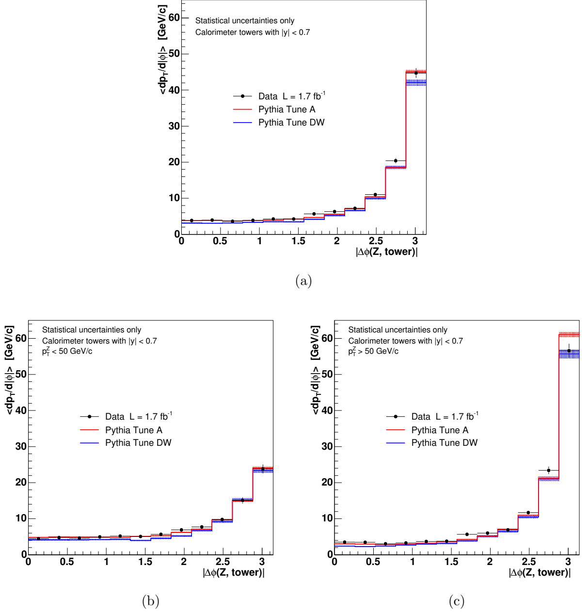
Figure 5.8: (a) Energy flow of the central calorimeter towers in Z/\gamma^*(\rightarrow e^+e^-) + \text{jets} events compared to the predictions from PYTHIA-TUNE A and TUNE DW. (b) Energy flow in events with p_T^Z < 50 \text{ GeV/c} and (c) events with p_T^Z > 50 \text{ GeV/c} . Only statistical uncertainties are included in the plots.
