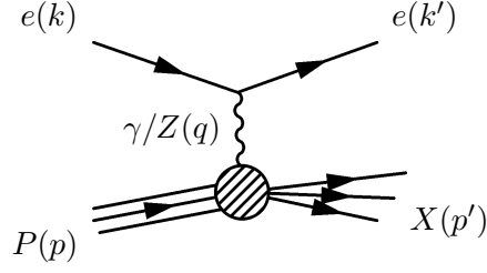
Figure 2.2: Schematic view of a deep inelastic scattering event: the photon (or a Z boson) interacts with a parton inside the proton.
