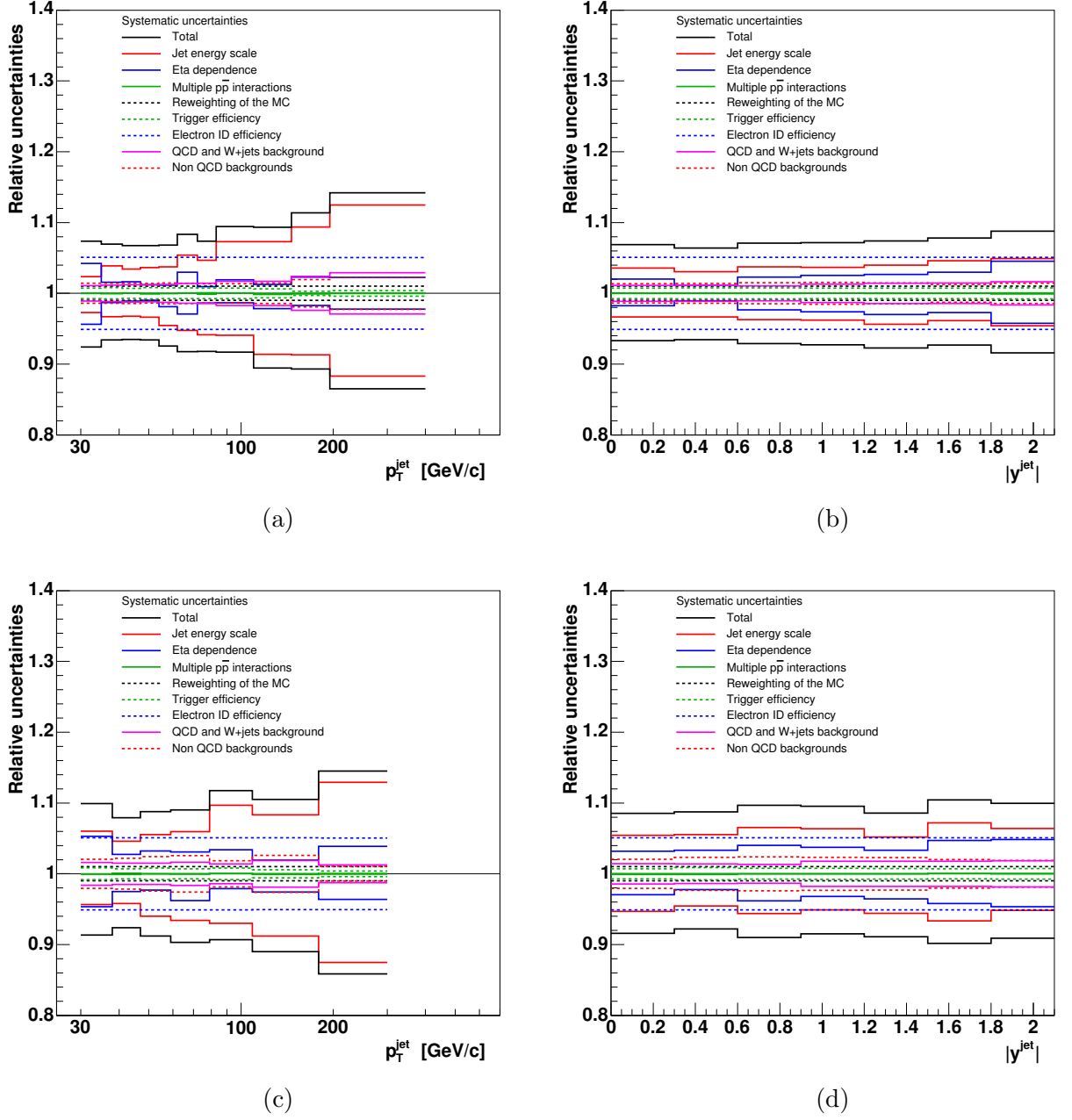
Figure 4.15: Total systematic uncertainties on the (a) p_T^{\text{jet}} and (b) y^{\text{jet}} inclusive jet differential cross sections in Z/\gamma^*(\rightarrow e^+e^-) + \geq 1 jet production. Total systematic uncertainties on the (c) p_T^{\text{jet}} and (d) y^{\text{jet}} inclusive jet differential cross sections in Z/\gamma^*(\rightarrow e^+e^-) + \geq 2 jets production.
