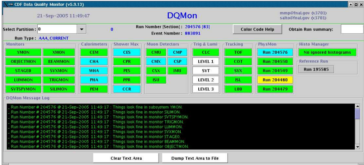
Figure A.1: DQMMon panel displays the status of some monitors and the results of the checks performed in the data from several subsystems.
