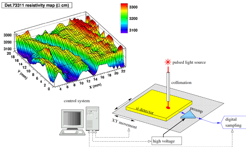
Fig. 3. In the upper left-hand side, a resistivity map of an FZ silicon detector is reported. The map has been obtained with the apparatus shown in the lower right-hand side of the picture. For details, see [7].
