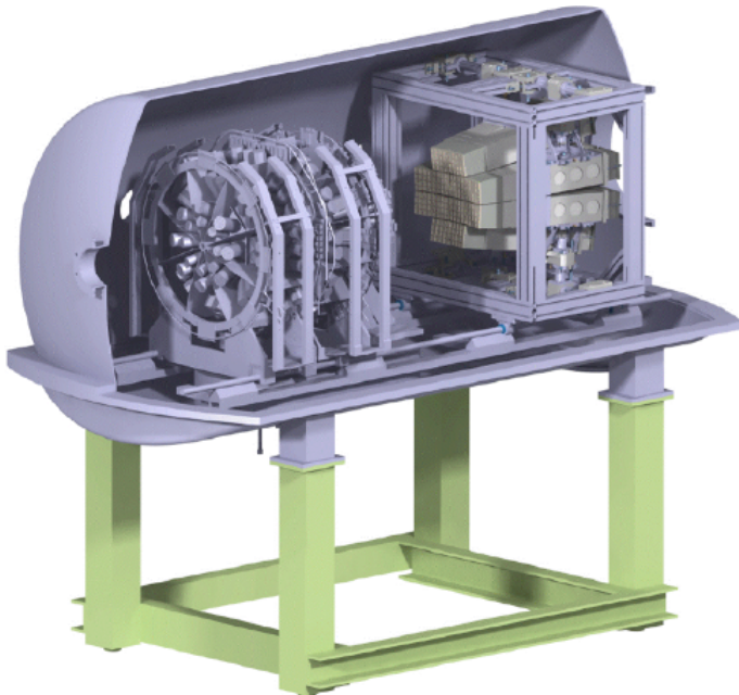
Fig. 8. The FAZIA Demonstrator coupled to INDRA multidetector. The system will begin commissioning by 2017.
