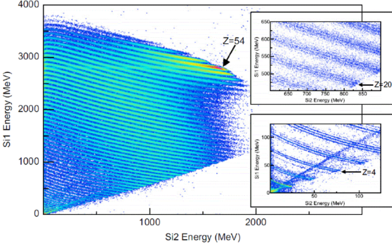
Fig. 5. \Delta E – E correlation using two FAZIA silicon detectors. The insets represent expansions around Z = 4 and Z = 20 . From [1].
