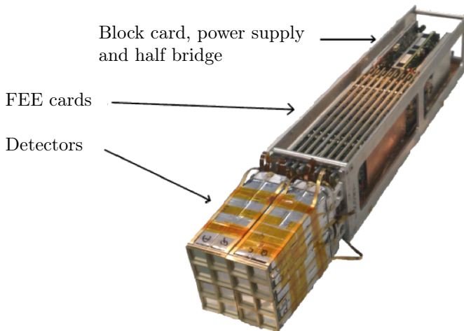
Fig. 7. The FAZIA Demonstrator. In the figure, one of the 12 blocks of the Demonstrator is shown, containing 16 telescopes and all the relevant FEE and ancillary electronics.
