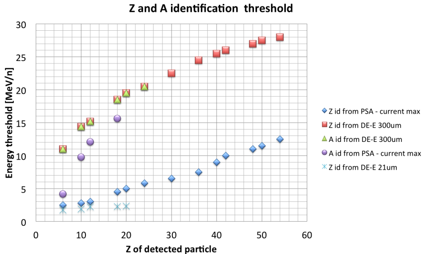
Fig. 6. Energy thresholds for Z and A identification of FAZIA detectors. For details, see the text.
