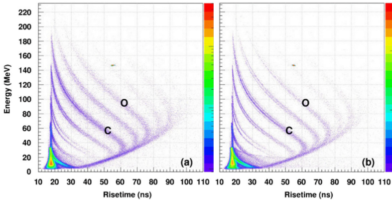
Fig. 2. Pulse shape identification obtained by plotting the energy of a stopped particle in the silicon detector as a function of the risetime of the charge signal. Parts (a) and (b) differ for crystal cut orientation, as described in the following and in [3].
