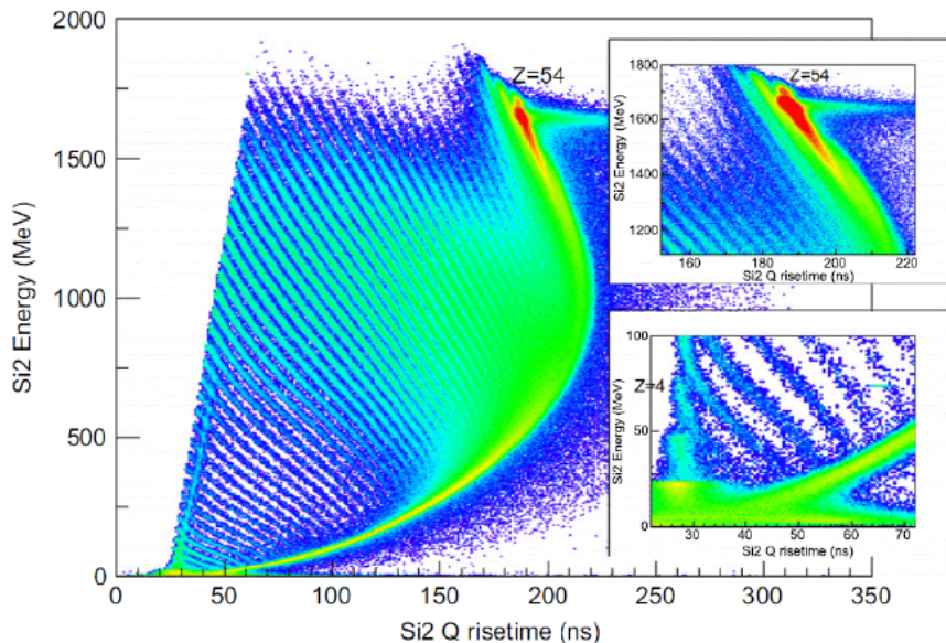
Fig. 4. PSA correlation: energy vs. rise-time of charge signal for nuclear fragments stopped in a FAZIA silicon 300 \mu\text{m} thick. In the insets, expansions of the regions of light particles and elastic scattering are reported. From [1].
