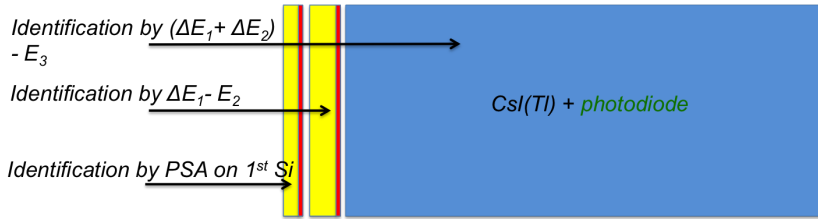
Fig. 1. The basic FAZIA module. The arrows represents particles of different energies which are identified in the way reported over the relevant arrows.
