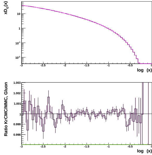
Fig. 3. Evolution of the gluon PDF from 1 GeV to 1000 GeV with \alpha(k_T) , rapidity ordering and minimal cut-off \lambda on k_T . No quark–gluon transitions.
