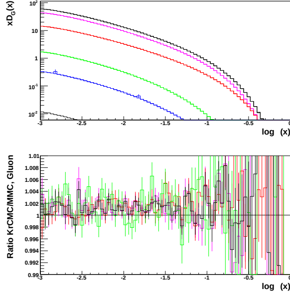
Fig. 5. Evolution of the gluon PDF from 1 GeV to 1000 GeV with \alpha(k_T) , rapidity ordering, minimal cut-off \lambda on k_T and quark–gluon transitions. Curves in the top frames correspond respectively (from upper to lower) to total distribution, and its components with 0,1,2,3 and 4 transitions.
