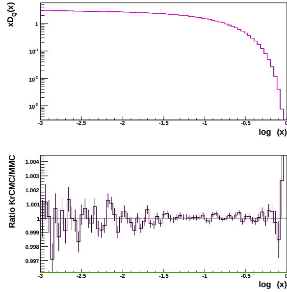
Fig. 4. Evolution of the quark PDF from 1 GeV to 1000 GeV with \alpha(k_T) , rapidity ordering and minimal cut-off \lambda on k_T . No quark–gluon transitions.
