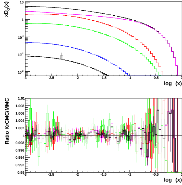
Fig. 6. Evolution of the quark PDF from 1 GeV to 1000 GeV with \alpha(k_T) , rapidity ordering, minimal cut-off \lambda on k_T and quark–gluon transitions. Curves in the top frame correspond respectively (from upper to lower) to total distribution, and its components with 0,1,2,3 and 4 transitions.
