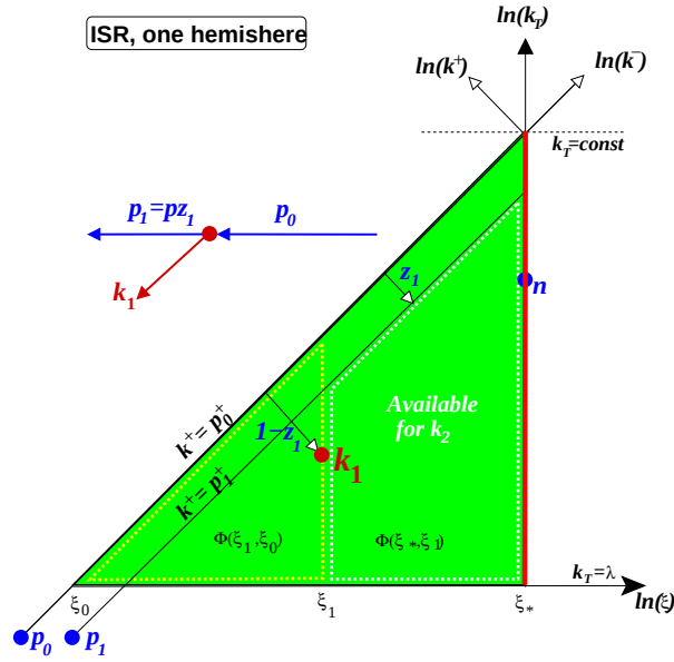
Fig. 1. Sudakov phase space of a single emission ordered in rapidity \eta = \log \xi and with minimal cut-off \lambda on k_T .
