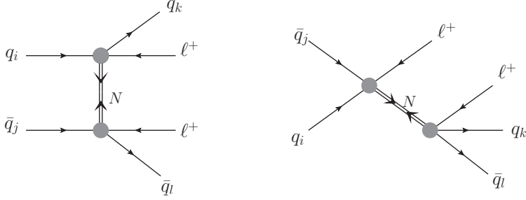
Figure 2: On the left the process with the exchange of a virtual heavy Majorana neutrino ( N ), on the right the process with resonant production of N and its subsequent decay.
