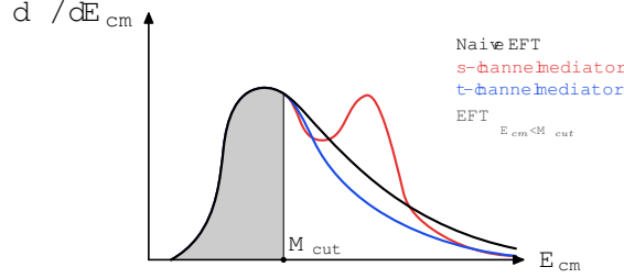
Figure 1: Schematic representation of the differential cross section for a two-to-two process in two Simplified Models (red and blue lines) and in the corresponding EFT.
