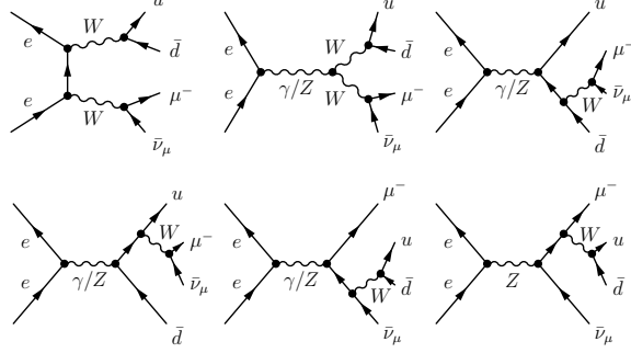
Figure 2: Diagrams contributing at tree-level to the e^-e^+ \rightarrow u\bar{d}\mu^-\bar{\nu}_\mu process.
