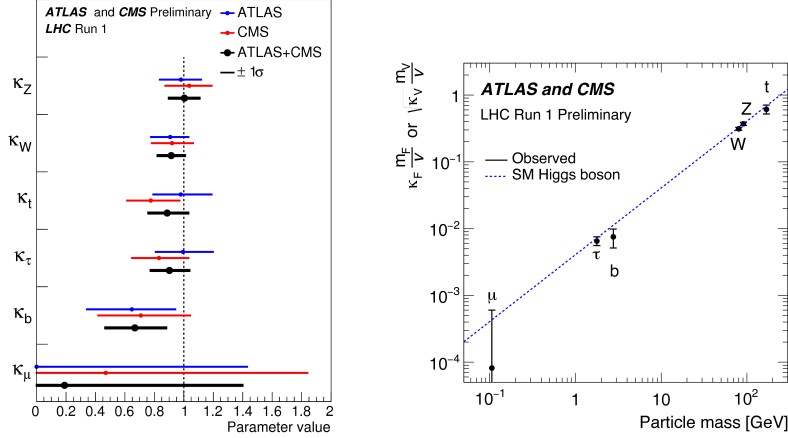
Figure 3: Results of the coupling modifier fit to the data of ATLAS, of CMS and on the combination of the two experiments. The left plot reports directly the best values of the coupling modifiers, the right plot reports the adimensional couplings entering the lagrangian. The linear dependence shows the property of the Higgs boson couplings to scale with the mass of the particle.
