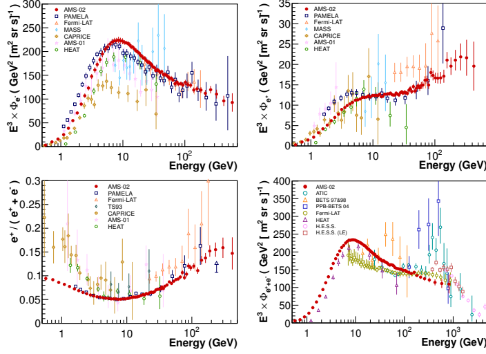
Figure 2: In red, AMS measurements of the e^- flux (top-left), of the e^+ flux (top-right), of the positron fraction (bottom-left) and of the (e^+ + e^-) flux (bottom-right). References in [2, 3, 5].
