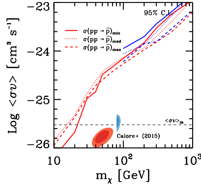
Figure 2: Antiproton bounds on DM annihilation rate. Red lines: b\bar{b} channel for NFW profile for different assumption for the secondary \bar{p} production. Blue lines: the same for the WW channel. The results obtained with a gNFW profile are indistinguishable from the NFW ones.
