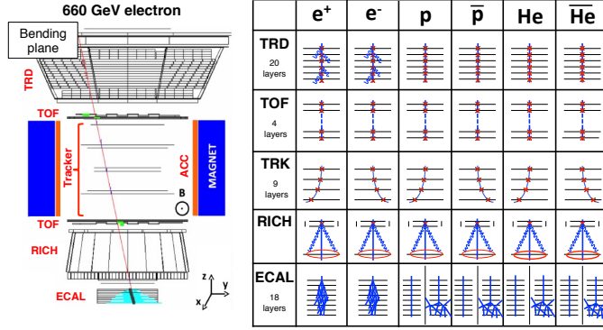
Figure 1: Left – Event display of a 660 GeV e^- detected by AMS-02. Right – Response of the AMS-02 subdetectors for different matter/antimatter CRs.
