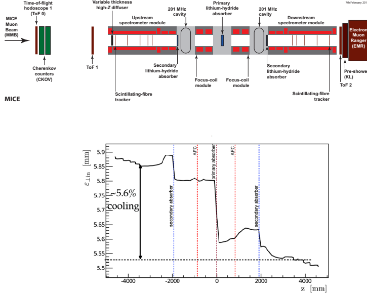
Figure 2: Top panel: view of the MICE experiment at RAL (for more details see 16 ). The cooling channel is put between two magnetic spectrometers 13 ) and two TOF stations 14 ) to measure particle parameters. Bottom panel: evolution of the 4D emittance in the MICE ionization-colling demo lattice, for a 6\pi \cdot \text{mm} , 200 MeV/c muon beam.
