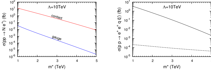
Figure 1: a) ^{12}\text{C} Production cross section of pp \rightarrow Ne^+ for gauge and contact interactions at \sqrt{s} = 13 \text{ TeV} , with CTEQ6m parton distribution functions and factorization scale \hat{Q} = m_N = m^* b) Comparison between the parton-level cross sections of the processes with resonant production of heavy Majorana neutrino and its subsequent decay (solid line) and that with the exchange of a virtual heavy Majorana neutrino (dashed line).
