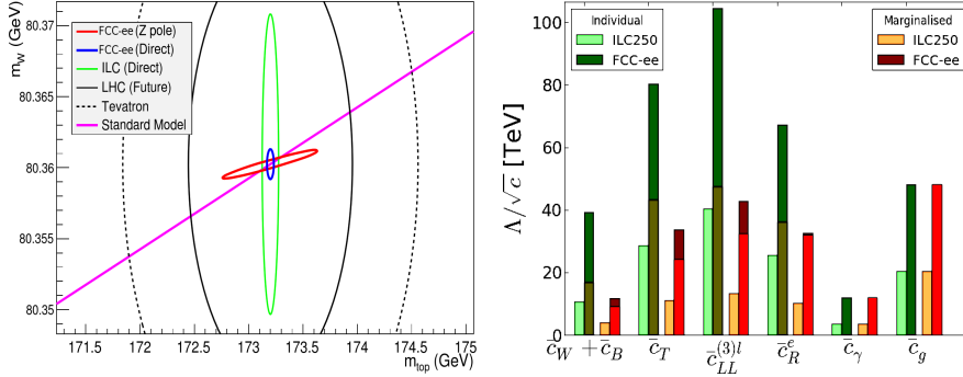
Figure 2: Left: 68% C.L. limits in the m_t - m_W plane at FCC-ee and other colliders 1) . Right: Energy reaches for dim-6 operators sensitive to EWPT, obtained from precision measurements at FCC-ee and ILC 11) .
