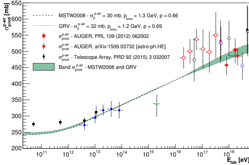
Figure 3: p - air production cross-section as deduced from the mini-jet model of 6) and 9), and its comparison with cosmic ray data. The band indicates uncertainties due to low- x behavior of the PDFs.
