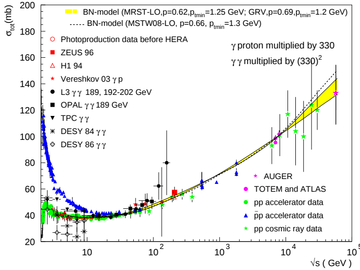
Figure 1: pp , p\bar{p} , \gamma p and \gamma\gamma total cross-sections, normalized to the same scale. The figure is from 1) .
