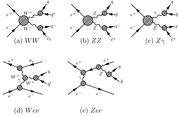
Figure 1: Classification of signatures in four-fermion production.
