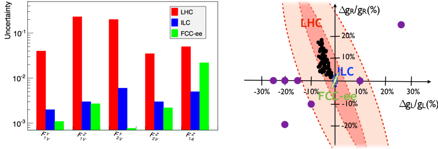
Figure 1: Statistical uncertainties on the axial and vector form factors expected at the LHC-13 with 300\text{ fb}^{-1} , at ILC-500 with 500\text{ fb}^{-1} and at FCC-ee-360 with 2.6\text{ ab}^{-1} (left panel). Typical deviations of the Zt_L\bar{t}_L and Zt_R\bar{t}_R couplings for various NP models (purple points) and for the 4DCHM (black points) together with the sensitivity expected at LHC-13 with 300 and 3000\text{ fb}^{-1} , outer and inner red lines, from ILC-500, blue dashed lines, and FCC-ee green lines (see 1) and refs. therein.)
