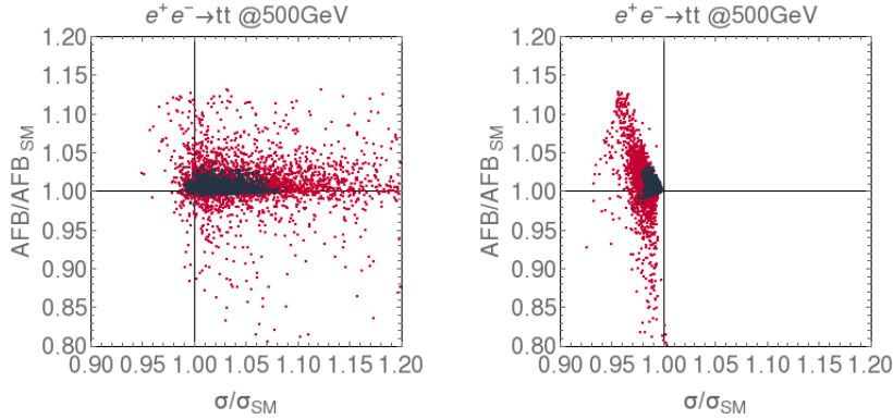
Figure 2: Predicted deviations for the cross section versus AFB for the process e^+e^- \rightarrow t\bar{t} with \sqrt{s} = 500 GeV without (left) and with (right) the inclusion of the \rho s present in the 4DCHM as propagating particles in the production diagrams. The points correspond to f = 0.75\text{--}1.5 TeV, g_\rho = 1.5\text{--}3 and a scanning over the fermion parameter. Blue points are compliant with current EW precision data and LHC measurements.
