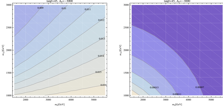
Figure 1: Contours of \delta_{23}^{QLL} (left) and \delta_{23}^{ULR} (right) in the m_0 - m_{1/2} plane for \tan \beta = 45 and A_0 = -3000 GeV in the CMSSM.
