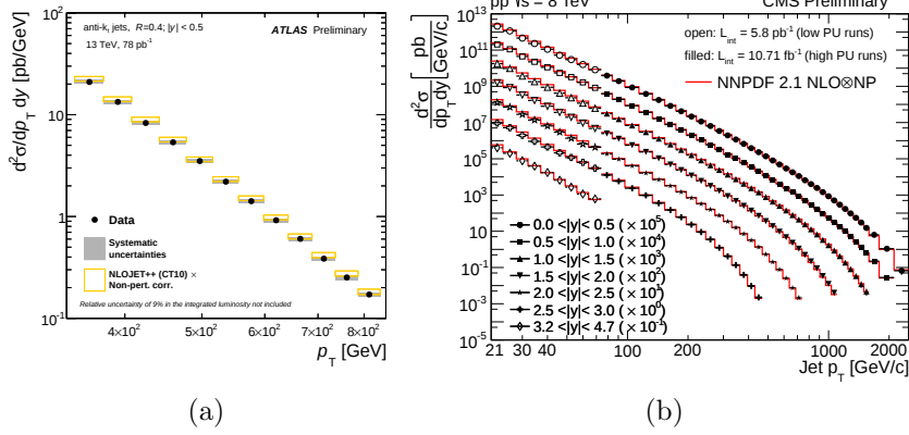
Figure 1: (a) jet cross section in |y| < 0.5 at \sqrt{s} = 13 TeV by ATLAS. (b) jet cross section in several |y| regions at 8 TeV by CMS.
