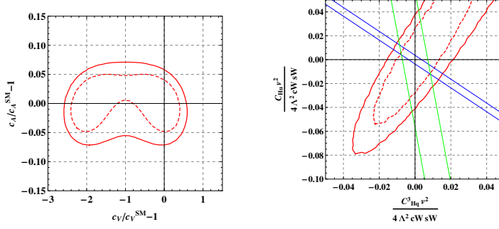
Figure 2: Left -68,95% credibility contours for the deviations of the (c_V, c_A) couplings. Right - credibility contours for the Wilson coefficients (C_{Hu}, C_{Hq}^3) ; on the top, the current constraints the electroweak precision tests (blue: \Delta T , green: \Delta\epsilon_B ) are presented.
