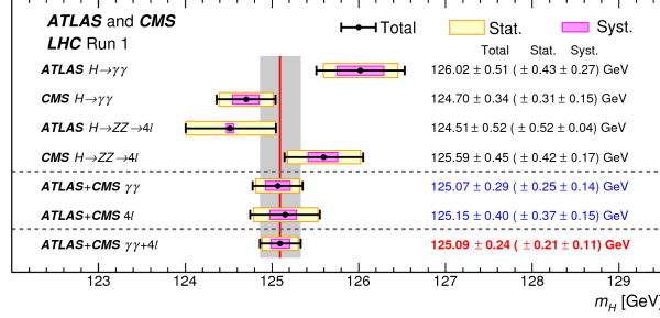
Figure 1: Summary of the results of the Higgs mass measurement for the two high resolution channels, namely \gamma\gamma and ZZ \rightarrow 4\text{leptons} . The combinations of ATLAS and CMS for each channel together with the global combination are also shown.
