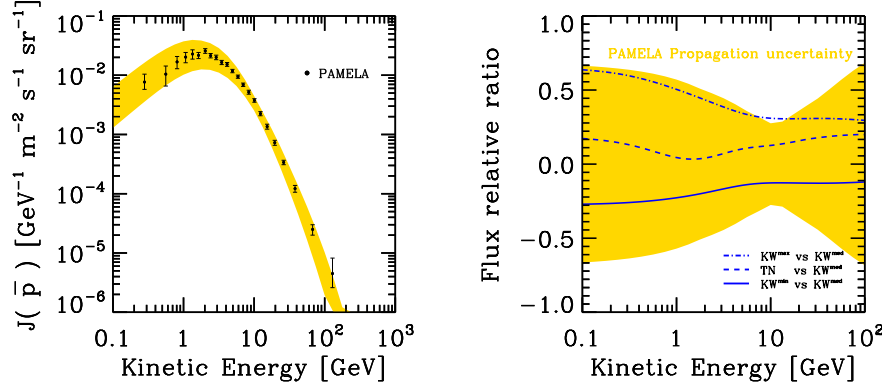
Figure 1: Left plot: The envelope of the secondary \bar{p} spectra computed with the different propagation models found to reproduce the B/C and primary spectra is compared with PAMELA data. Right plot: Comparison between propagation and nuclear uncertainties. Yellow band: Error on the \bar{p} flux due to the uncertainty in the propagation parameters. Blue lines: The relative difference between the \bar{p} flux computed using the fiducial CS used in this work and its maximal/minimal realization; a comparison is also done with the model conventionally adopted in the related literature (solid line).
