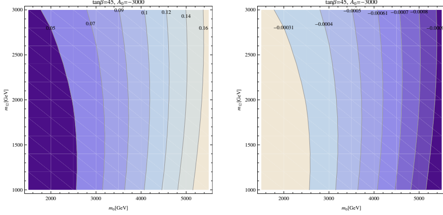
Figure 2: Contours of \Delta M_W^{\text{MFV}} in GeV (left) and \sin^2 \theta_{\text{eff}} in the m_0 - m_{1/2} plane for \tan \beta = 45 and A_0 = -3000 GeV in the CMSSM.
