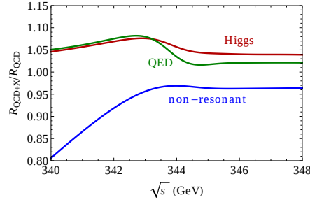
Figure 3: Relative size of the different non-QCD corrections to the top-pair production cross section with respect to the pure QCD result at \mu = 80 \text{ GeV} . Figure from 10) .
