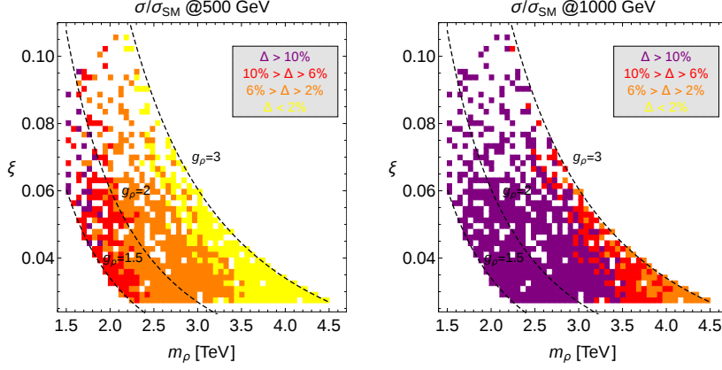
Figure 3: Predicted deviations for the cross section of the process e^+e^- \rightarrow t\bar{t} at 500 and 1000 GeV in the 4DCHM compared with the SM as functions of m_\rho = fg_\rho and \xi = v^2/f^2 . For each point we have selected the configuration yielding the maximal deviation defined as \Delta = (\sigma^{4\text{DCHM}} - \sigma^{\text{SM}})/\sigma^{\text{SM}} . The points correspond to f=0.75\text{-}1.5 TeV, g_\rho=1.5\text{-}3 . All points are compliant with EW precision data and current LHC measurements.
