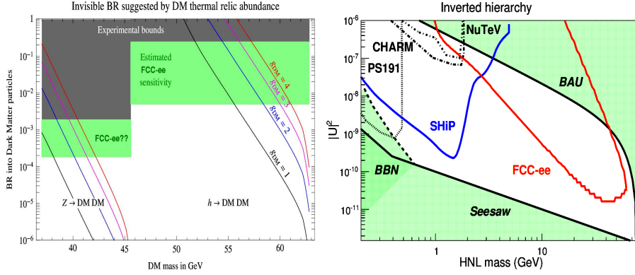
Figure 4: Regions of sensitivity of FCC-ee for: (i) Z and H decays into DM in the \text{BR}_{Z,H \rightarrow \text{DM DM}} vs. m_{\text{DM}} plane (left) 16) , and (ii) sterile neutrinos as a function of their mass and mixing to light neutrinos (inverted hierarchy) for 10^{12} Z decays (right) 17) .
