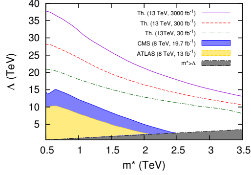
Figure 3: expected 3- \sigma contour plots at RunII from heavy composite Majorana neutrino compared to current bounds from CMS and ATLAS searches of excited leptons in RunI.
