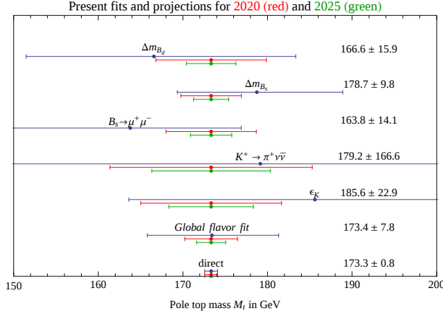
Figure 2: Summary of present and future determinations of M_t from flavour data. For future projections, we have fixed the central value of M_t to the present direct measurement.
