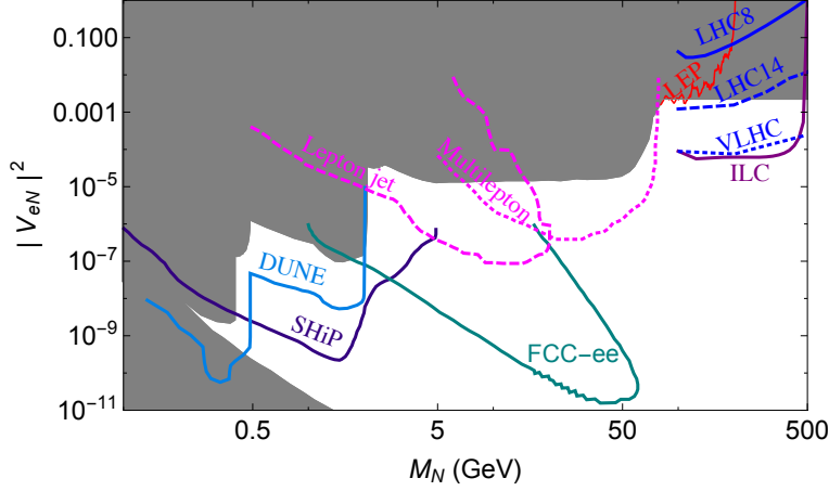
Figure 1: Current (shaded) and future limits in the heavy neutrino mass-mixing plane for the electron flavor. For details and for limits in other flavors, see 4, 7 ).
