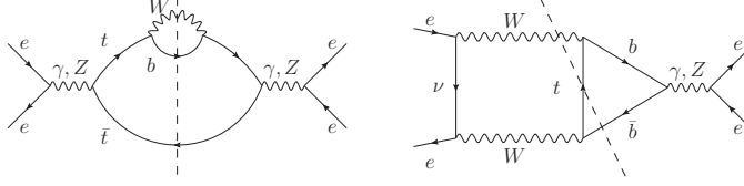
Figure 1: Sample diagrams for the nonresonant production of the W^+W^-b\bar{b} final state.
