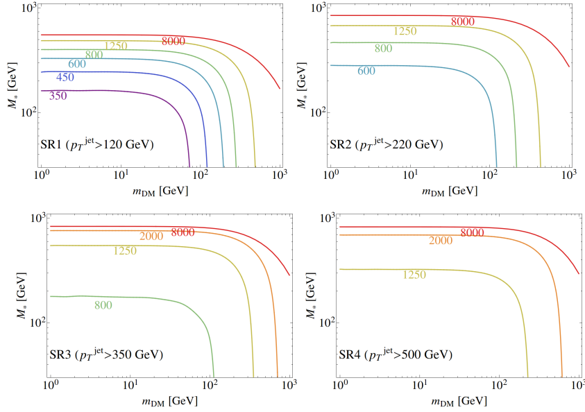
Figure 2: Lower exclusion bounds on M_* as a function of m_{\text{DM}} for different values of M_{\text{cut}} , reported in the plots with the same colour of the corresponding lines. The four plots correspond to the four signal regions of 3) .
