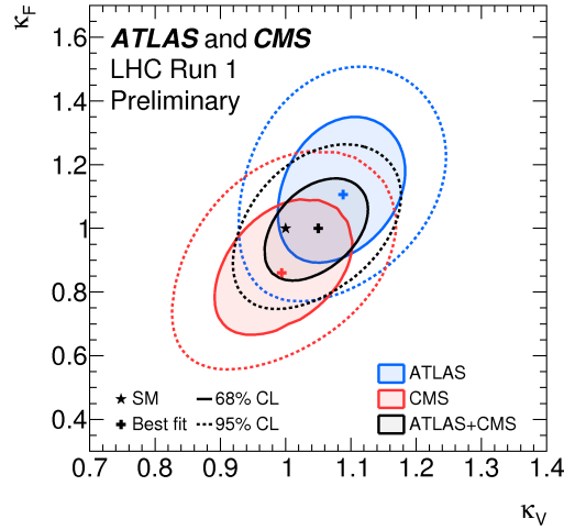
Figure 4: Result of the two parameter fit with two overall coupling modifiers to fermions and to vectors, \kappa_F and \kappa_V as free parameters. Results are shown for ATLAS, for CMS and for the combination of the two experiments.
