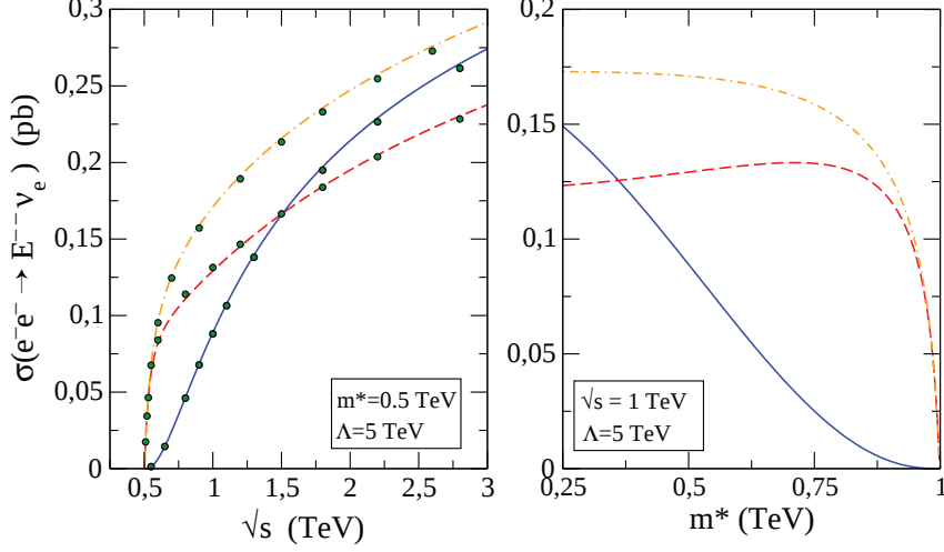
Figure 1: The total cross sections for the process e^-e^- \rightarrow E^{--}\nu_e is shown. In the left panel the total cross section against the center of mass energy is displayed for the different isospin multiplets. The solid blue line stands for E^{--} \in I_W = 1 , the dashed red (orange dot-dashed) curve for E^{--} \in I_W = 3/2 with (without) the interference contribution taken into account. The right panel shows the total cross section against mass. The compositeness parameters are set to ( m^* = 0.5 TeV, \Lambda = 5 TeV). The green dots show the CalcHEP output.
