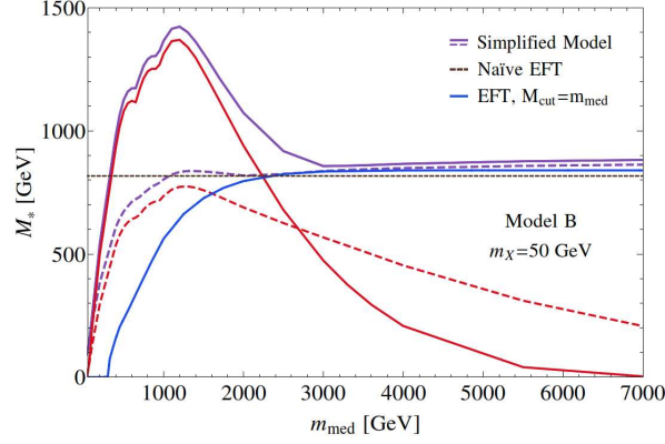
Figure 4: Exclusion limits on M_* as function of the mediator mass \tilde{m} for m_X = 50 GeV. The blue line shows the recasting, in the Simplified Model, of the limit obtained within the truncated EFT. The purple lines are obtained in the full Simplified Model, while the red ones represent the limit obtained by using the subset of simulated events where the mediator was resonantly produced. Solid and dashed lines correspond to two different values of the mediator width, respectively \tilde{m}/(8\pi) and \tilde{m}/3 .
