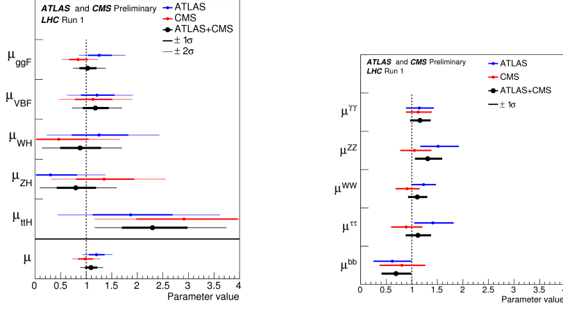
Figure 2: Results of the signal strength fit to the data of ATLAS, of CMS and on the combination of the two experiments. (left) production signal strengths and (right) decay signal strengths.
