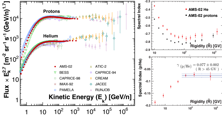
Figure 3: Left – in red, AMS measurements of the p and He fluxes as function of the kinetic energy per nucleon. Right – Spectral index rigidity dependence of the p and He fluxes (top) and of the p/He ratio (bottom). References in 8) .
