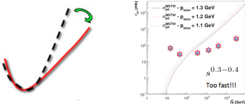
Figure 2: At left a cartoon describing the transformation of the initial fast rise of the cross-section, compatible with a power-law, into a smooth asymptotic behavior, compatible with a logarithmic behavior. At right the energy behavior of a QCD cross-section compared with a typical hadronic cross-section (stars).
