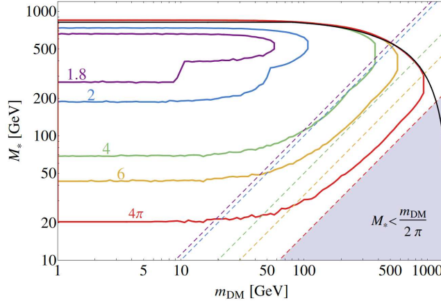
Figure 3: Combined exclusion limits on M_* as function of m_{\text{DM}} for different values of g_* , reported in the plots with the same colour of the corresponding lines. The areas below the dashed lines correspond to the regions where M_* < 2m_{\text{DM}}/g_* , where the value of g_* is the one corresponding to the colour of the dashed line. Within those regions, the condition (1) for the validity of the EFT is automatically violated.
