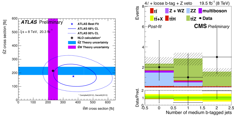
Figure 2: a) Result of the combined two-dimensional simultaneous fit to the t\bar{t}W and t\bar{t}Z cross sections along with the 68% and 95% CL uncertainty contours. The shaded areas correspond to 14% uncertainty, which includes renormalisation and factorisation scale uncertainties as well as and PDF uncertainties including \alpha_s variations. b) Post-fit plots of the final discriminant for the four leptons t\bar{t}Z channel with exactly one lepton pair consistent with a Z \rightarrow l^+l^- decay,
