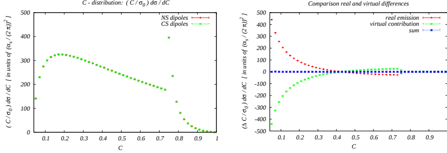
Figure 1: Left: Total result for differential distribution \frac{C}{\sigma_0} \frac{d\sigma^{\text{NLO}}}{dC} using both our dipoles (red, "NS") and Catani-Seymour dipoles (green, "CS"). The standard literature result obtained using the CS scheme is completely reproduced with the NS dipoles. Right: Differences \Delta_{\text{CS-NS}} for real emission (red, upper) and virtual (green, lower) contributions, showing that especially for low C values the contributions in the two schemes significantly differ. Adding up \Delta^{\text{real}} + \Delta^{\text{virt}} renders 0 as expected.
