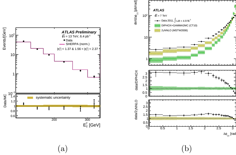
Figure 2: (a) E_T^\gamma distribution from inclusive photon at 13 TeV by ATLAS and (b) \Delta\phi_{\gamma\gamma} distribution from diphoton at 7 TeV by ATLAS.
