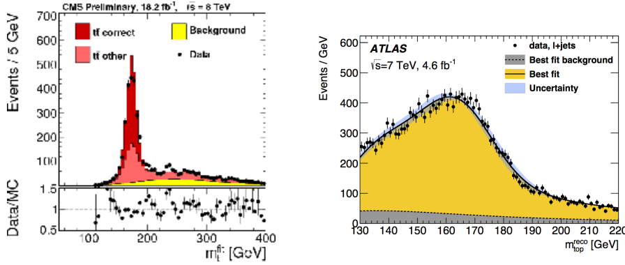
Figure 1: a) Reconstructed m_t from the CMS kinematic fit. The simulated signal and the background from event mixing are normalized to the data b) Fitted ATLAS m_t distribution. The fitted probability density functions for the background alone and for signal-plus-background are also shown. The uncertainty bands indicate the total uncertainty on the signal-plus-background fit obtained from pseudo-experiments.
