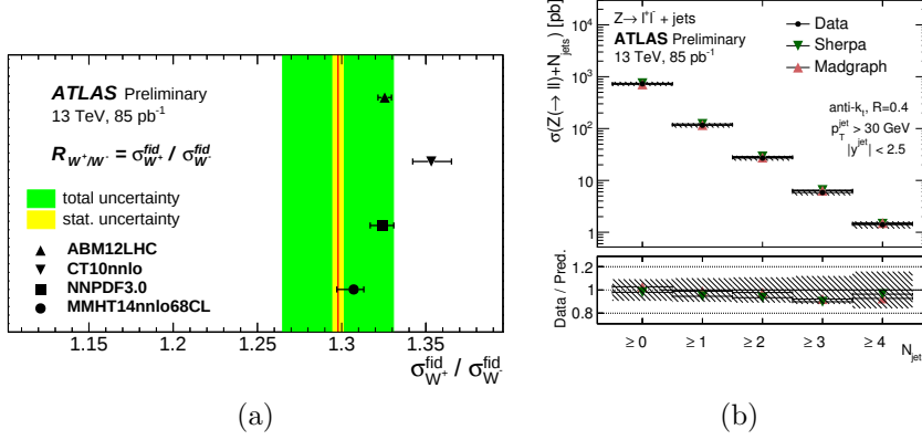
Figure 3: (a) ratio of W^+ and W^- cross section and (b) jet multiplicity in Z +jet by ATLAS at 13 TeV.
