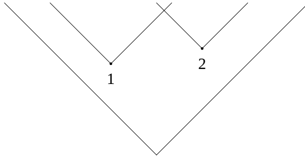
Figure 1.4: String breaking in two points.
