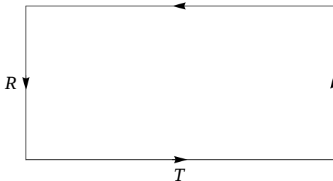
Figure 1.1: Rectangular Wilson loop.
