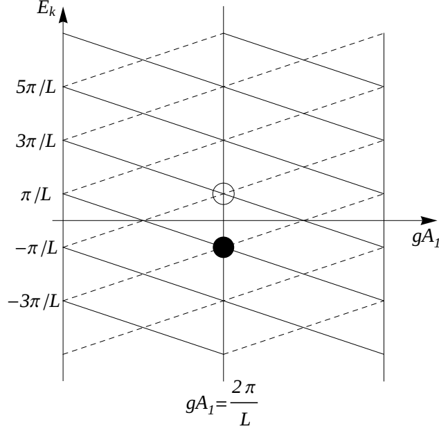
Figure 2.2: Level crossing in background electric field.
