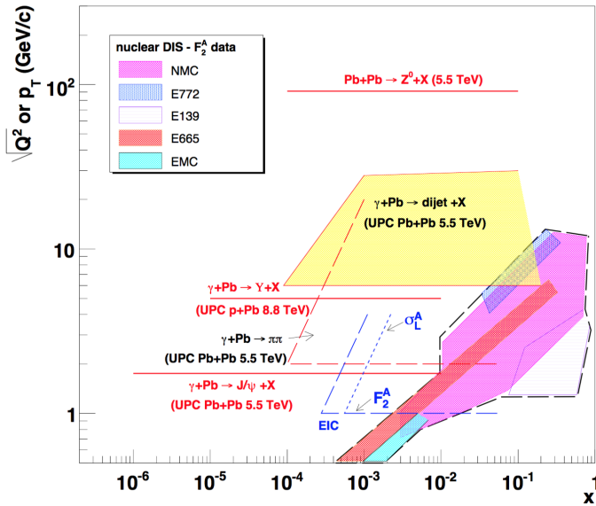
Fig. 4. The kinematic range in which UPCs at the LHC can probe gluons in protons and nuclei in quarkonium production, dijet and dihadron production. The Q^2 value for the typical gluon virtuality in exclusive quarkonium photoproduction is shown for J/\psi and \Upsilon . For comparison, the kinematic ranges for J/\psi at RHIC, structure function F_2^A and cross section \sigma_L^A at eRHIC and Z^0 hadron production at the LHC are also shown [2].
