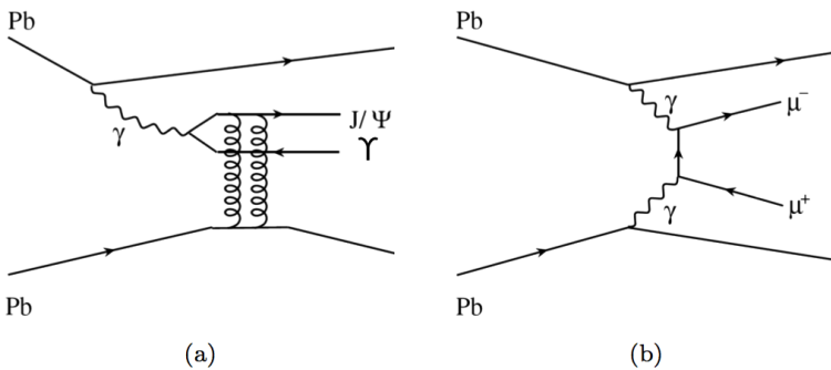
Fig. 2. The Feynman diagrams of an UPC for PbPb. Diagram (a) shows photoproduction process of vector mesons, (b) is a \gamma\gamma interaction producing two muons, the main background to the analysed process.
