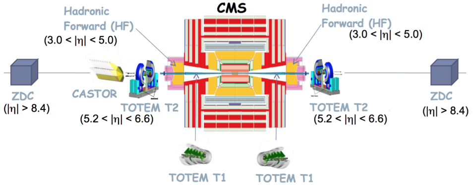
Fig. 5. Forward sub-detectors in the CMS. On both sides, there are HF calorimeters, TOTEM and ZDC detectors. CASTOR calorimeter is installed on one side only.
