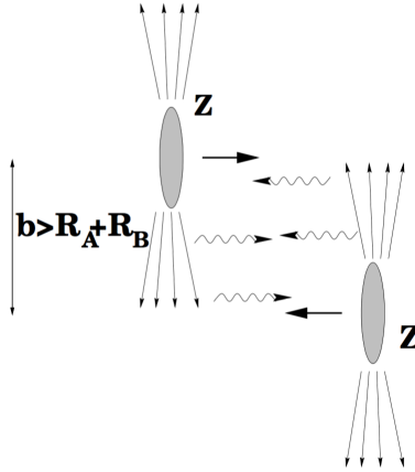
Fig. 3. A representation of an UPC. The pancake-like shape of the nuclei is due to the relativistic Lorentz contraction.
