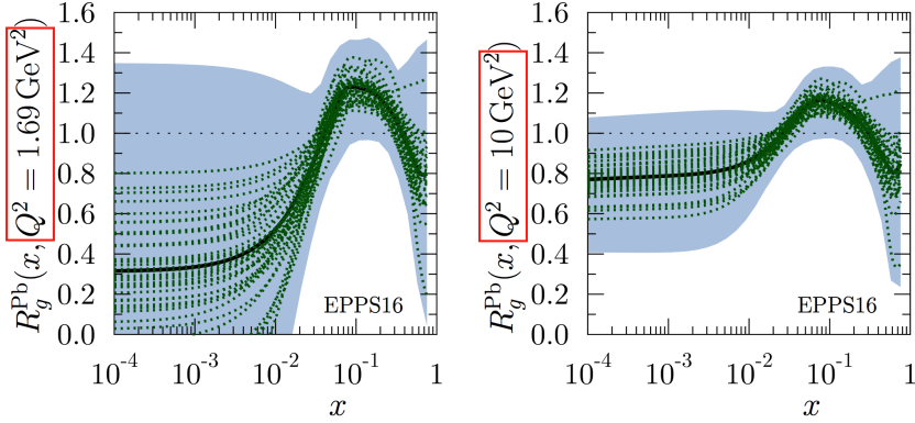
Fig. 1. The EPPS16 nuclear modifications for lead. Largest uncertainty for gluon distributions is for x < 10^{-2} and low Q^2 . This is because of a lack of data in this region. Dotted lines show different contributions to the uncertainties [1].
