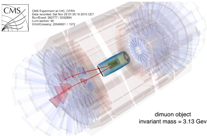
Fig. 6. The event display shows one of the selected events, the visualisation of the CMS detector can be seen, together with two trajectories of muons going into forward direction. The reconstructed invariant mass of the two leptons is about the J/\psi mass.
