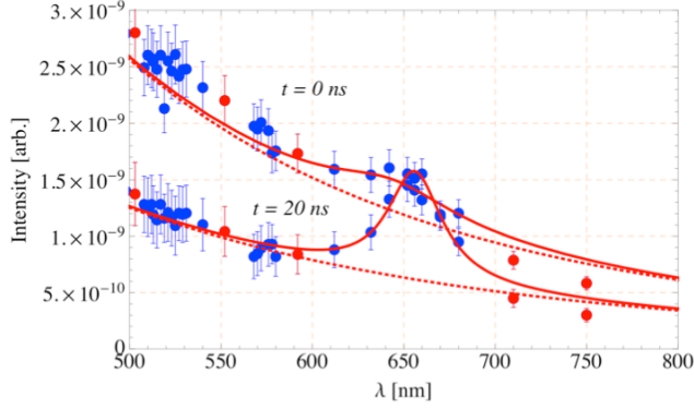
Fig. 5: Enlargement around H \alpha resonance from Figure 4. The dotted line is the blackbody curve and the solid line includes the Lorentz curve.
