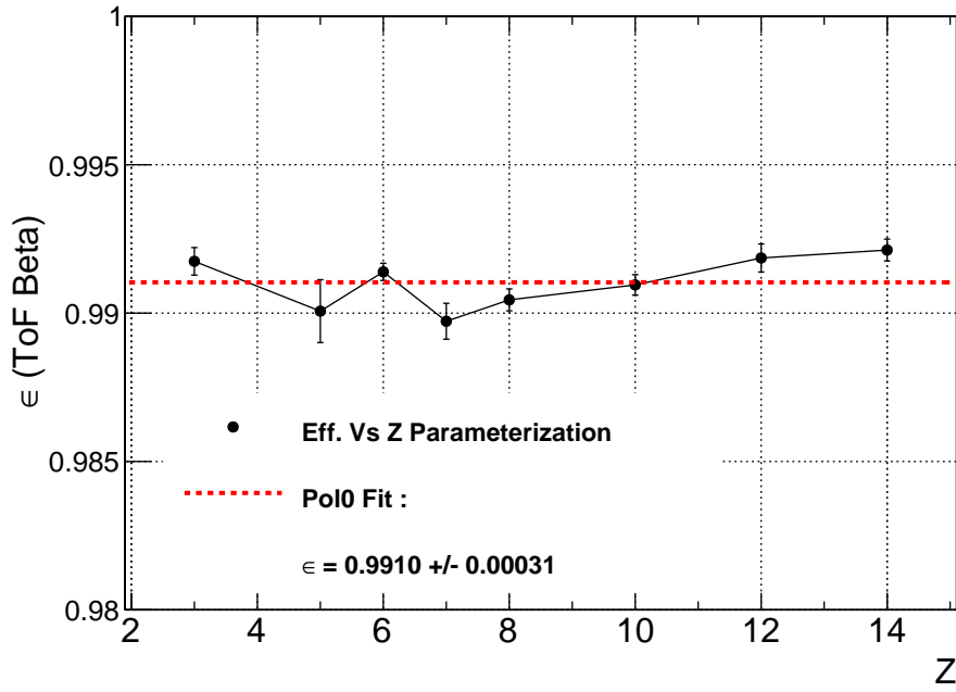
FIGURE 6.7 – Results of the constant parameterizations (black points) of the ToF beta reconstruction efficiency in function of the nuclear charge Z . Odd Z nuclei above nitrogen have been neglected. A single efficiency value for all nuclei is extracted based on a constant fit (dashed red line).
