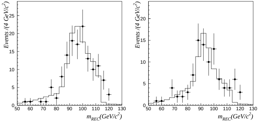
Fig. 13. The (reconstructed) mass distributions of the events passing the event filter in the ANN-based analysis (left) and the cut-based analysis (right) in the ALEPH Higgs boson searches in the year 2000 [6]. The background predictions are drawn with histograms and the data with error bars. A compatible number of excess events (Higgs event candidates) was found, observable as the excess of events in the high mass region.
