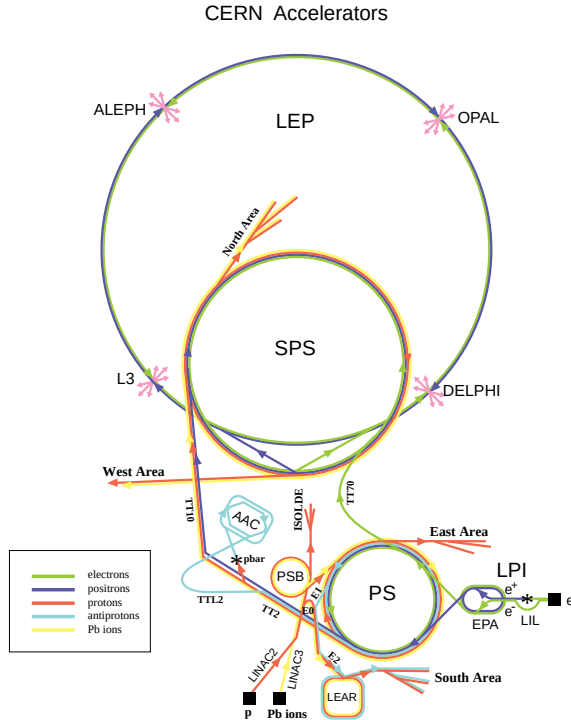
Fig. 1. The Large Electron Positron collider acceleration chain.
