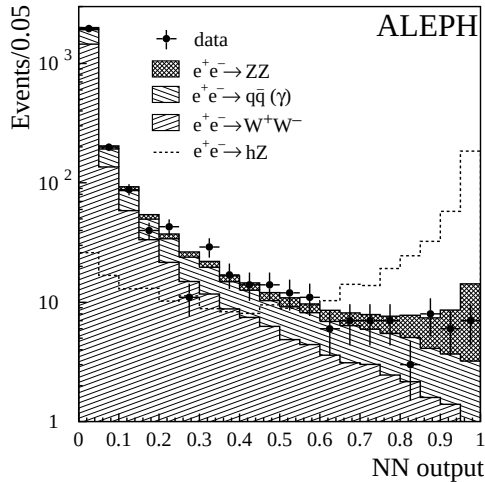
Fig.10. An example of the signal e^+e^- \rightarrow HZ^0 \rightarrow \dots probability distribution as given by an ANN for Monte Carlo simulated signal and background (histograms) and LEP data (error bars) in the Higgs boson searches at ALEPH.
