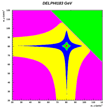
Fig. 7. Example of the expected PDF distribution of the masses of two W bosons produced in a e^+e^- \rightarrow W^+W^- \rightarrow \dots process. The shape is a star-like distribution originating in a product of two Breit–Wigner functions; the green area represents the kinematically inaccessible region. Clearly, cuts in terms of |m_1 - m_W| < \varepsilon \times |m_2 - m_W| < \varepsilon , which would result in a rectangular selected PDF region, would be far from optimal.
