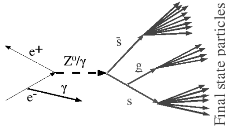
Fig. 4. A diagrammatic representation of a process e^+e^- \rightarrow Z^0/\gamma \rightarrow s\bar{s}g resulting in a similar final state topology as the above 'signal process, thus contributing as potential 'contamination' (background) source inside a selected data sample.
