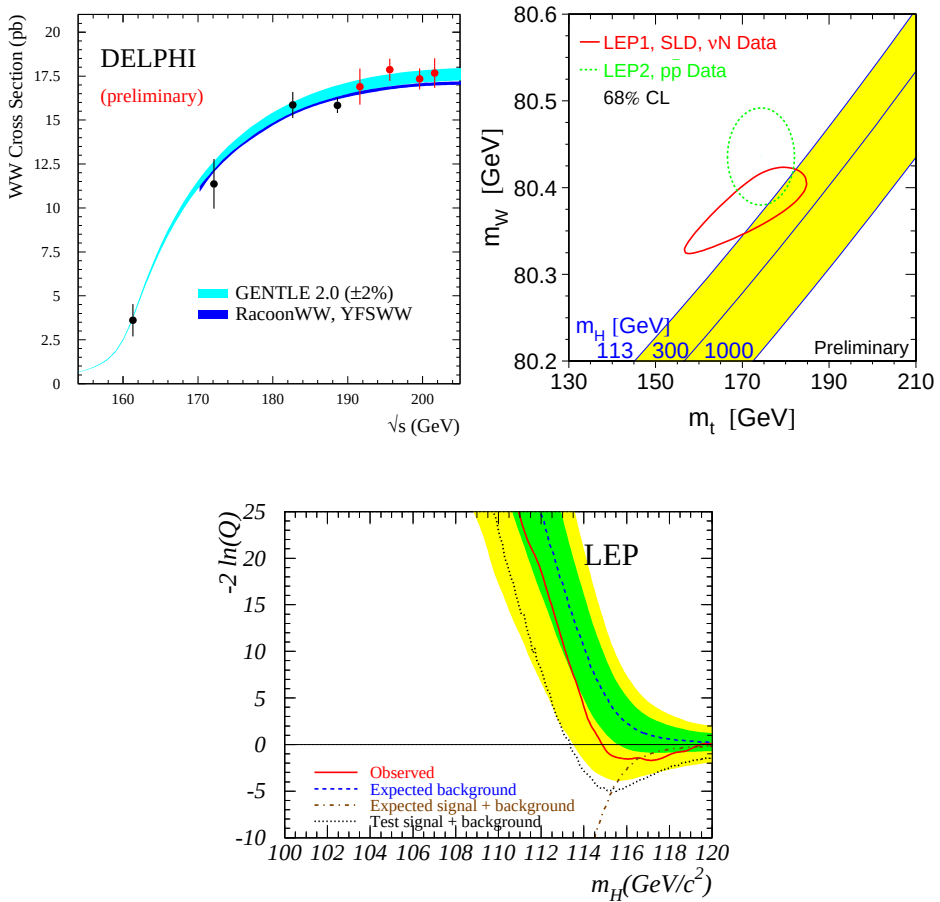
Fig. 2. Examples of fields of research at LEP: e^+e^- \rightarrow W^+W^- cross-section measurement [4] (left), Higgs boson mass constraints using the W boson and top quark mass measurements (right) and estimation of the Standard Model Higgs boson mass probability [5] (bottom) .
