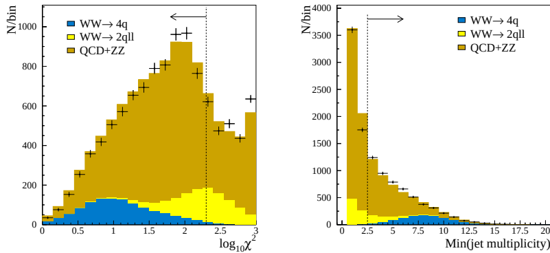
Fig. 6. Examples of two cuts applied on the data sample when trying to filter out the (four-jet) signal events e^+e^- \rightarrow W^+W^- \rightarrow 4q in presence of several background processes. The data is represented with error bars and the Monte Carlo predictions with histograms.
