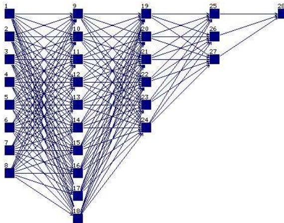
Fig.8. Example of a Artificial Neural Network layout presented by the SNNS package. One input layer on the left with three hidden layers and one neuron in the output layer is chosen, the neurons are chosen to be fully connected to the neighbouring layers.
