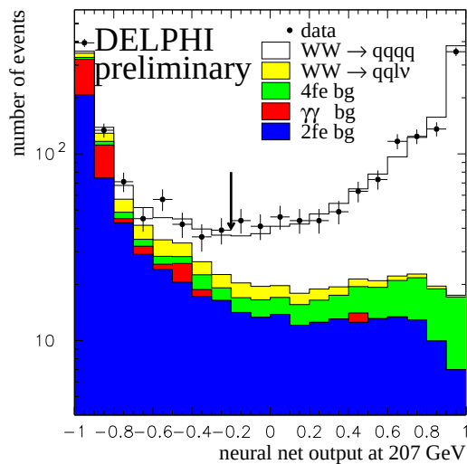
Fig. 9. An example of the signal probability distribution as given by an ANN for Monte Carlo simulated signal and background (histograms) and LEP data (error bars) as recorded at \sqrt{s} = 207 GeV by the DELPHI detector [4].
