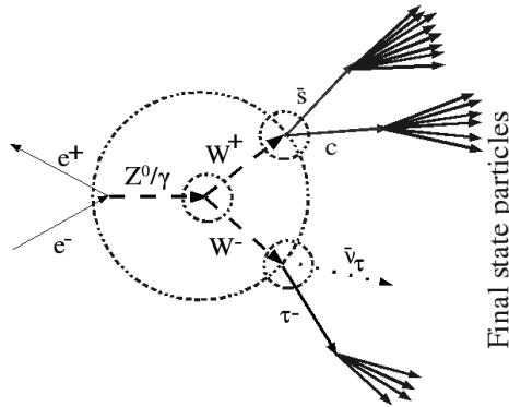
Fig.3. A diagrammatic scheme of the process e^+e^- \rightarrow Z^0/\gamma \rightarrow W^+W^- \rightarrow \bar{s}c\tau^-\bar{\nu}_\tau \rightarrow \dots . Possible regions/parameters of interest (resonances, couplings etc. ) are marked with dashed circles.
