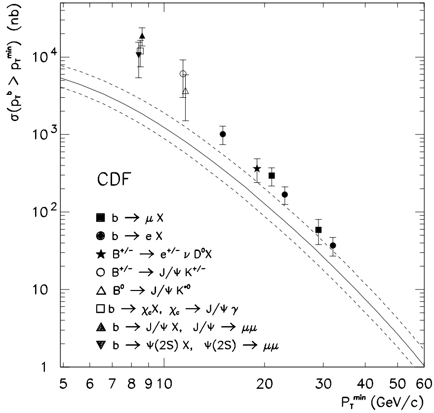
Figure 11.2: Integral b -quark production cross sections for |y^b| < 1 from the CDF experiment in p\bar{p} collisions at \sqrt{s} = 1.8 TeV.
