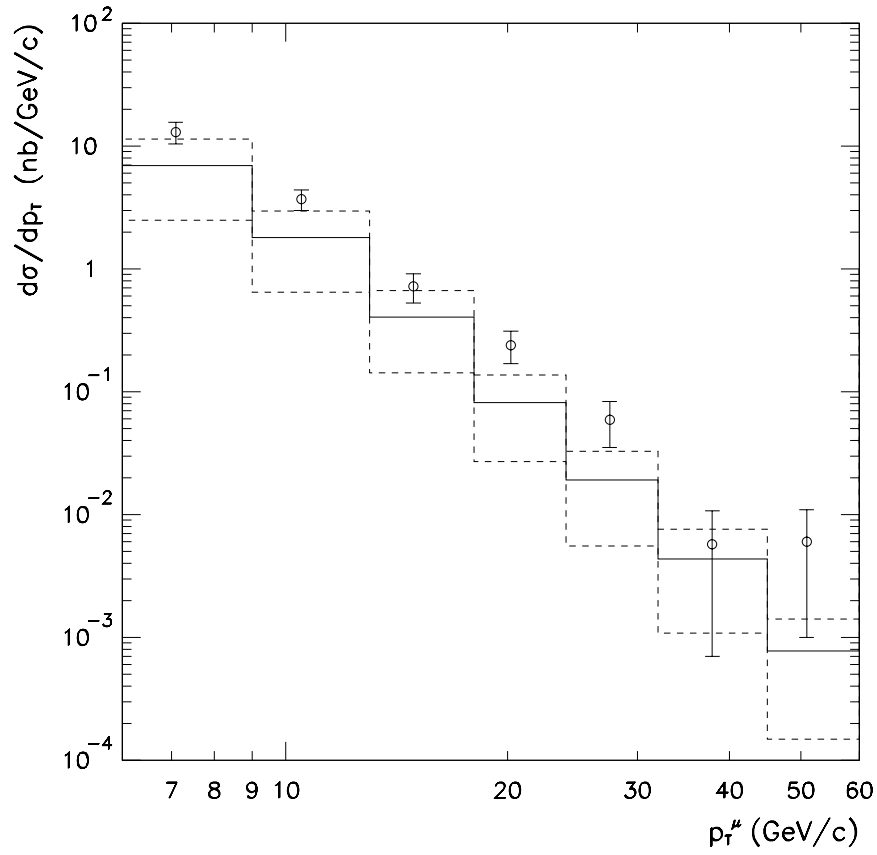
Figure 9.6: Muon spectrum for events with |\eta^\mu| < 0.8 and E_T^{\text{high}} > 15 \text{ GeV} with c , \pi/K and W/Z components subtracted, compared to a Monte Carlo calculation of b \rightarrow \mu X processes (solid histogram). The dashed histogram indicates the uncertainty in the Monte Carlo prediction.
