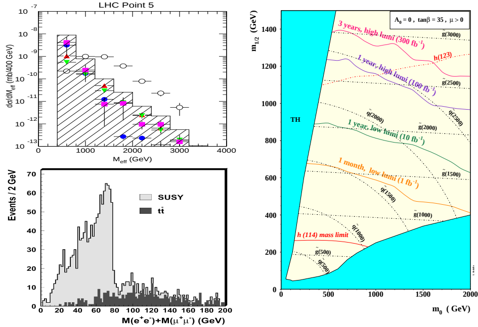
Fig. 5. Upper left: M_{\text{eff}} distribution for a mSugra benchmark point ( m_0 = 100 GeV, m_{1/2} = 300 GeV, A_0 = 0 , \tan\beta = 2 , \text{sgn}(\mu) = + ) signal and background obtained from a simulation of the ATLAS detector (from Ref. [8]). Lower left: invariant mass spectrum of two opposite-sign, same-flavor leptons from the decay \tilde{\chi}_2^0 \rightarrow \ell^+ \ell^- \tilde{\chi}_1^0 for 10 \text{fb}^{-1} of data simulated in the CMS detector (from Ref. [13]). Right: discovery region for the inclusive SUSY search in the (m_0, m_{1/2}) -plane of mSugra for integrated luminosities from 1 to 300 \text{fb}^{-1} (from Ref. [4]).
