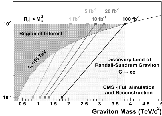
Fig. 6. Discovery reach in the parameter space of the Randall–Sundrum model of warped extra dimensions (from Ref. [19]).
