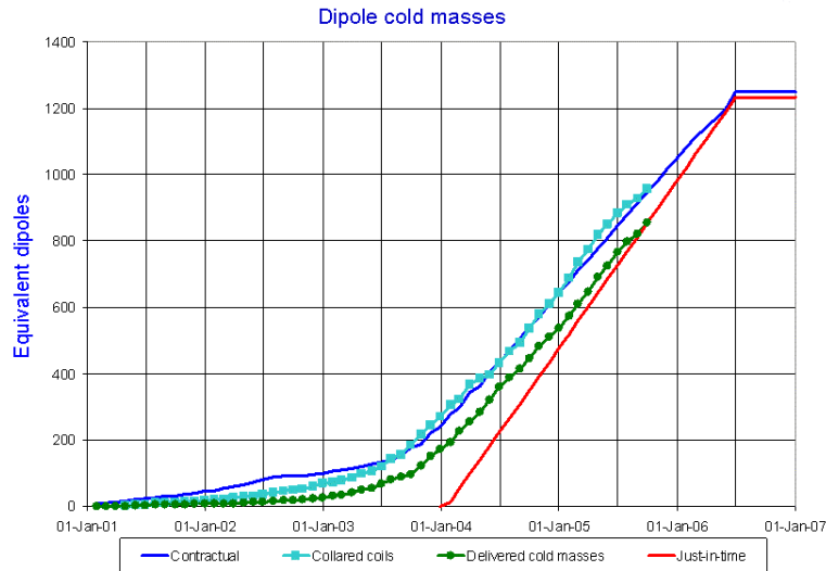
Fig. 1. Number of produced and delivered dipole cold masses for the LHC ring as of 30/09/2005 (from Ref. [1]).
