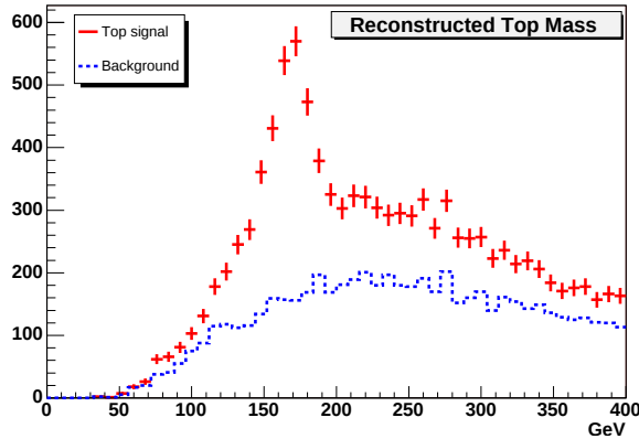
Fig. 3. Reconstructed three-jet invariant mass for semi-leptonic t\bar{t} events and expected background from W+4 jet events passed through a simulation of the ATLAS detector. The integrated luminosity is 150 \text{ pb}^{-1} and no b -tagging is applied (from Ref. [7]).
