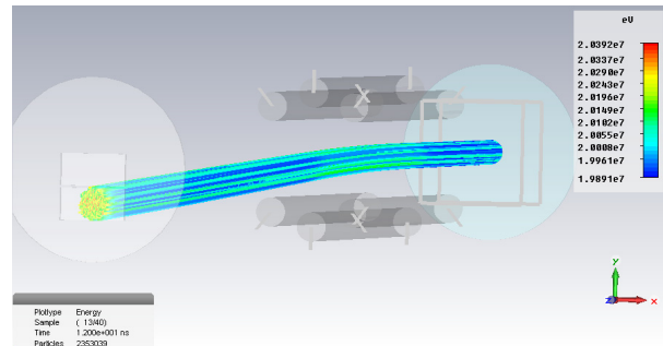
Figure 11: Beam dynamics simulation in CST.
