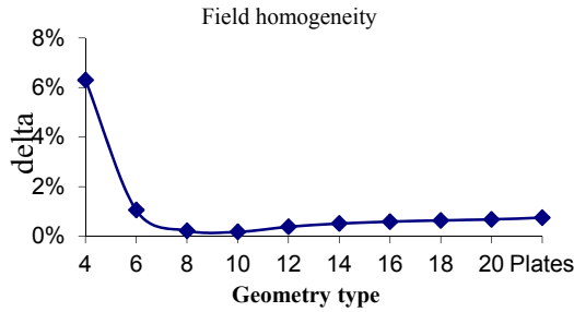
Figure 2: The dependence of field homogeneity from geometry type (total number of cylinders or plates).
