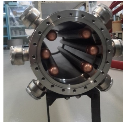
Figure 10: The kicker actual photo.
