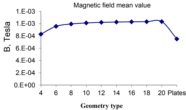
Figure 3: The dependence of magnetic field mean value from geometry type (total number of cylinders or plates).
