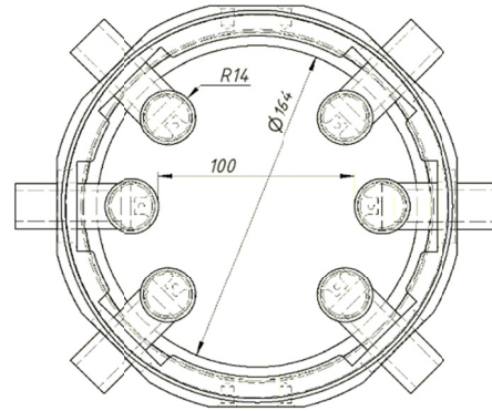
Figure 9: The kicker actual design (all dimensions are in mm).
