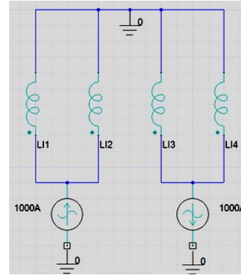
Figure 4: Simplified equivalent electrical circuit of the magnet.
