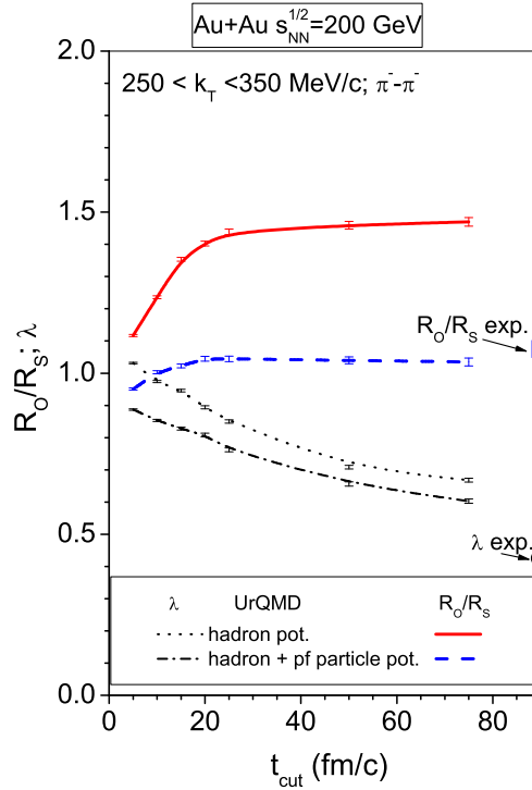
Fig. 4. Time evolution of the ratio R_O/R_S and the \lambda factor of pion source at 250 < k_T < 350 MeV/c, which are calculated with potentials for formed baryons and with potentials for both formed and “pre-formed” particles. The R_O/R_S and \lambda experimental data are represented by a square and a circle at the right end of the plot.
