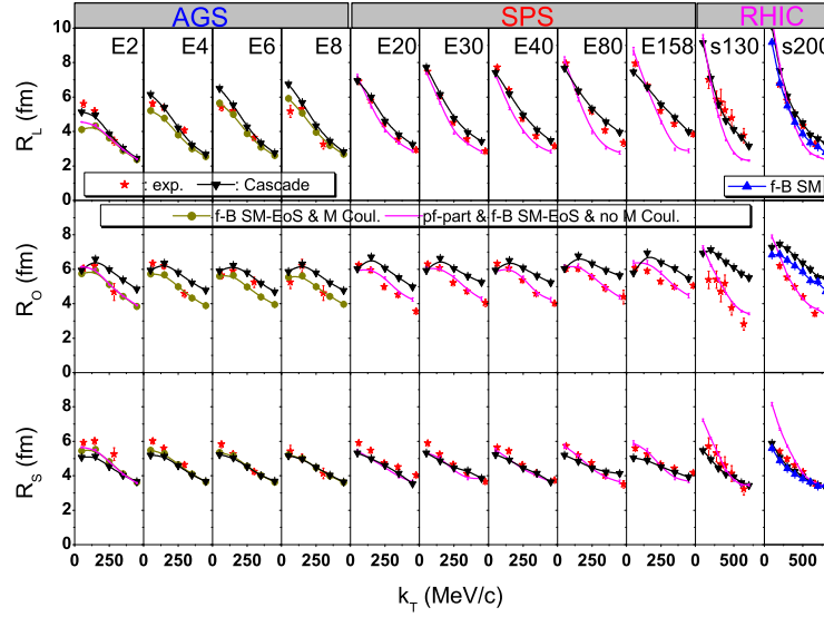
Fig.1. k_T dependence of R_L , R_O , and R_S for central HICs at AGS, SPS, and RHIC energies. The data (solid stars) are from E895, NA49, STAR, and PHENIX collaborations [17–22]. The calculations with cascade mode and with potentials for confined baryons are shown by the lines with symbols. The results with potentials for both “pre-formed” particles and confined baryons but without Coulomb potential for mesons are shown by lines.
