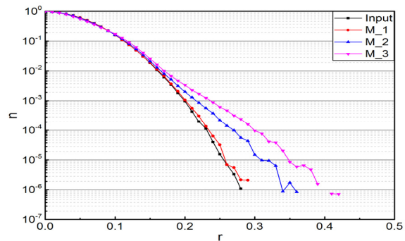
Figure 8: The phase space particle density at the end of the FODO line from multi-particle simulations for various mismatch parameters.
