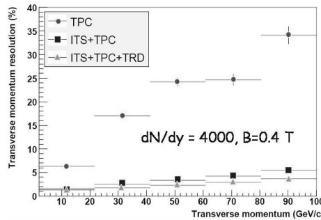
Fig. 4. Momentum resolution as a function of the transverse momentum.
