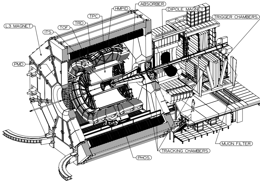
Fig. 1. Axonometric view of the ALICE layout.
