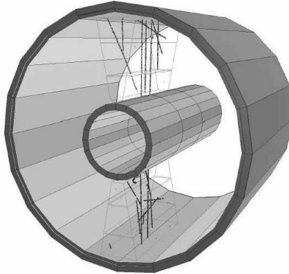
Fig. 6. Cosmic ray tracks reconstructed in two TPC sectors during the commissioning tests.
