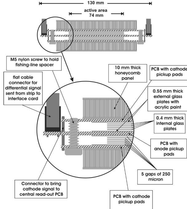
Fig. 5. Schematic description of the ALICE TOF.
