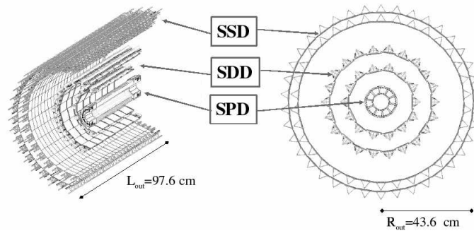
Fig. 2. Artist view of the six cylindrical layers of the Inner Tracking System.
