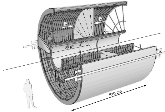
Fig. 3. Cut-away view of the ALICE TPC showing the central electrode and the field cage.
