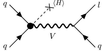
Fig. 2. Proton decay through a dimension five interaction for V = (3, 1)_{\frac{2}{3}} and V = (3, 3)_{\frac{2}{3}} .
