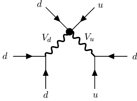
Fig. 3. Process mediating n - \bar{n} oscillations via the vector diquark (6, 2)_{-1/6} .
