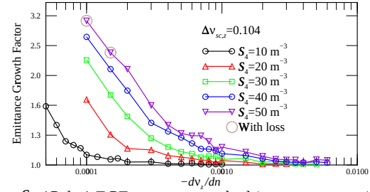
Figure 6: (Color) EGF across octupole driven resonance 4\nu_{x0} = 27 versus tune-ramp rate for various octupole strengths after 70-turn injection. Linear relationships are evident.
