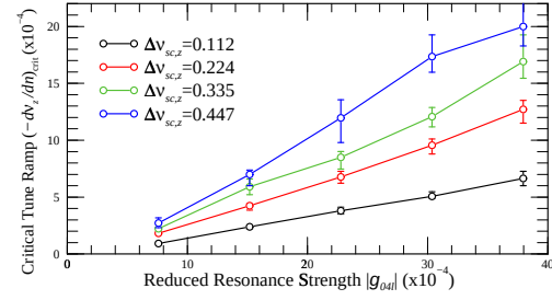
Figure 7: (Color) Critical tune-ramp rate across the octupole driven resonance 4\nu_{z0} = 27 versus reduced resonance strength |g_{04\ell}| for various bunch intensities.
