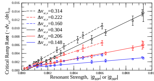
Figure 4: (Color) Critical tune-ramp rate across the systematic 6th-order resonances versus reduced resonance strength |g_{60P}| or |g_{06P}| for various linear space-charge tune shifts or bunch intensities. Dashed and solid lines are linear fits to the data.
