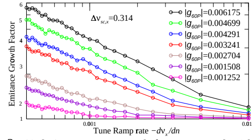
Figure 3: (Color) Emittance growth factor across the 6th-order systematic resonance 6\nu_{x0} = P versus tune-ramp rate for various resonance strengths |g_{60P}| at 100-turn injection.
