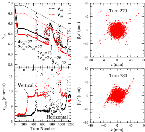
Figure 5: (Color) After 70-turn injection of 4 \times 10^{11} per turn, bare tunes are ramped downwards at 0.0005 per turn (top-left). Emittance growths are seen (bottom-left) while crossing various parametric resonances, usually accompanied by beam loss. Right: vertical phase-space distributions at turns 270 (top) and 780 (bottom), demonstrating the crossing of 4\nu_{z0} = 27 and 2\nu_{z0} = 13 .
