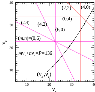
Figure 1: (Color) Tune diagram of Ruggiero's proposed FFAGs, showing the crossing of the systematic 4th and 6th-order resonances in a ramp cycle (arrowed curve).
