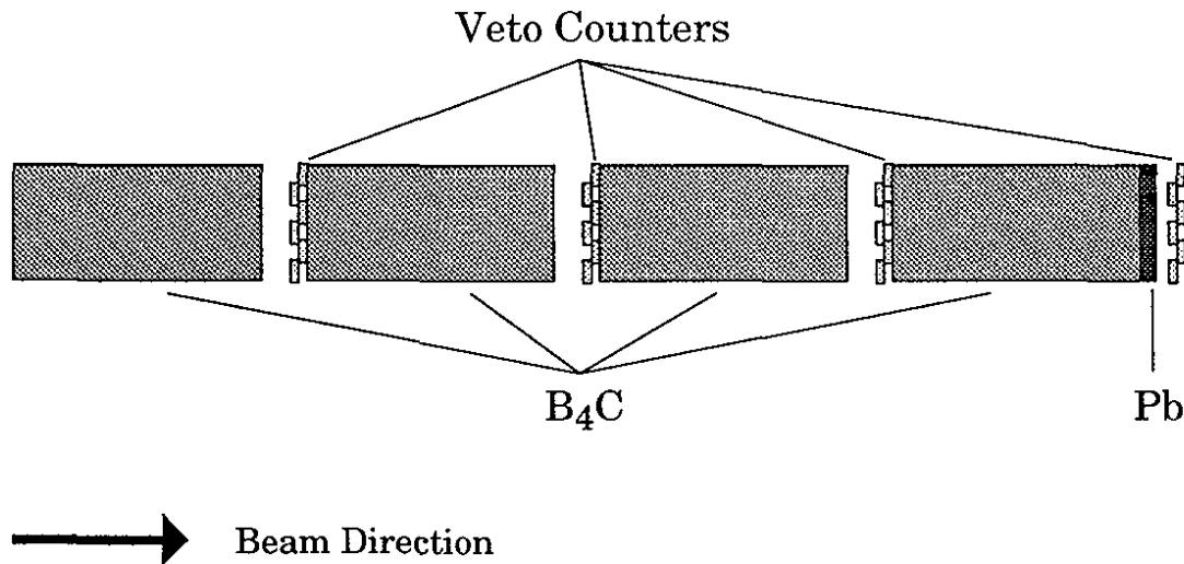
Figure 8. The makeup of the regenerator.
