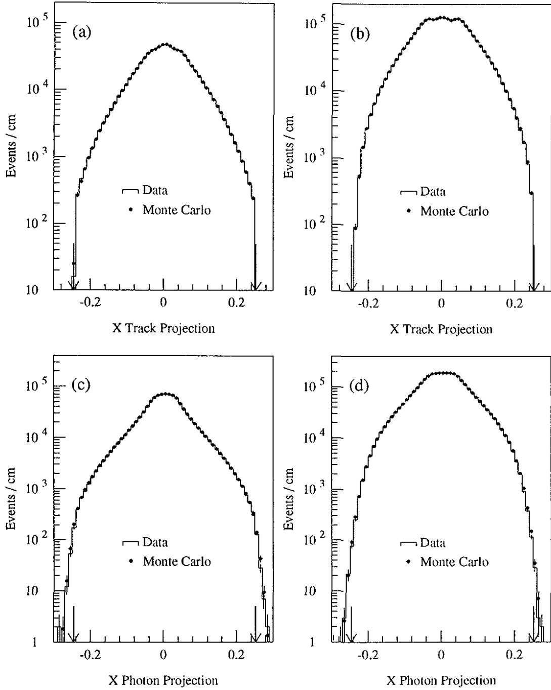
Figure 82. \pi^+\pi^- track illumination and 2\pi^0 photon illumination in the x view at the plane of the HDRA for data and Monte Carlo simulation. (a) Vacuum beam \pi^+\pi^- track projection. (b) Regenerator beam \pi^+\pi^- track projection. (c) Vacuum beam 2\pi^0 photon projection. (d) Regenerator beam 2\pi^0 photon projection. The arrows indicate the locations of the HDRA edges.
