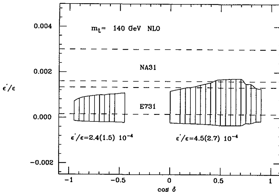
Figure 143. Variation of Re(\epsilon'/\epsilon) vs \cos \delta in the calculation of the Rome group [103]. The experimental 1 standard deviation bands for this result and the preliminary NA31 result indicated by the dashed lines. The top mass used in the calculation was 140 \text{ GeV}/c^2 . Plot courtesy L. Reina.
