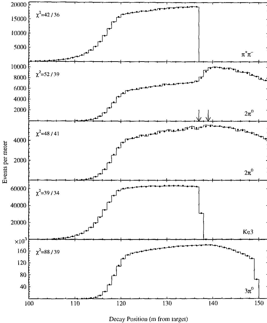
Figure 109. The vacuum beam z distributions in data and Monte Carlo simulation for the \pi^+\pi^- , 2\pi^0 , Ke3 and 3\pi^0 kaon decay modes. The two 2\pi^0 subsets with and without the lead sheet are shown separately. The \chi^2 for the z for the overlay is listed for each distribution. All other cuts have been applied. For the 3\pi^0 overlay, 52 units of \chi^2 come from the 4 z bins at 116 to 120 m, where the data is most sensitive to an energy scale mismatch. The arrows shown for the lead sheet 2\pi^0 lead sheet subset indicate the z region excluded from the analysis.
