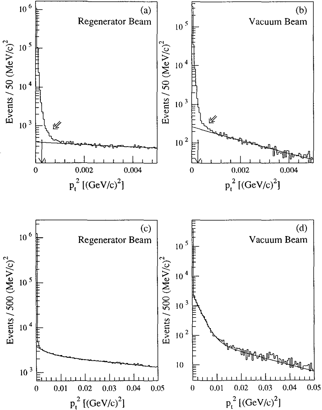
Figure 48. p_t^2 distribution for \pi^+\pi^- candidates after all other cuts are applied for two different ranges of p_t^2 . Parts (a) and (b) show the distribution out to 5000 (MeV/c) 2 for the regenerator and vacuum beams, respectively. At this scale, the structure of the coherent peak, the location of the analysis cut (vertical arrow) and the radiative tail from \pi^+\pi^-\gamma decays are all visible. Parts (c) and (d) show the distribution out to 50,000 (MeV/c) 2 for the regenerator and vacuum beams, respectively, where the contributions from different background sources (see text) are more apparent. In all four parts, solid line is the best fit to the overall background shape.
