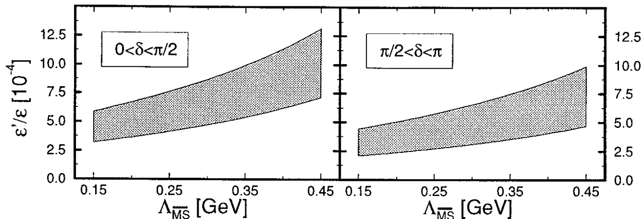
Figure 144. Variation of Re(\epsilon'/\epsilon) as a function of \Lambda_{\overline{MS}} in the calculation of the Munich group [104]. The bands are shown for the allowed region in the first and second quadrants of the \rho - \eta plane. Plot courtesy M. Jamin.
