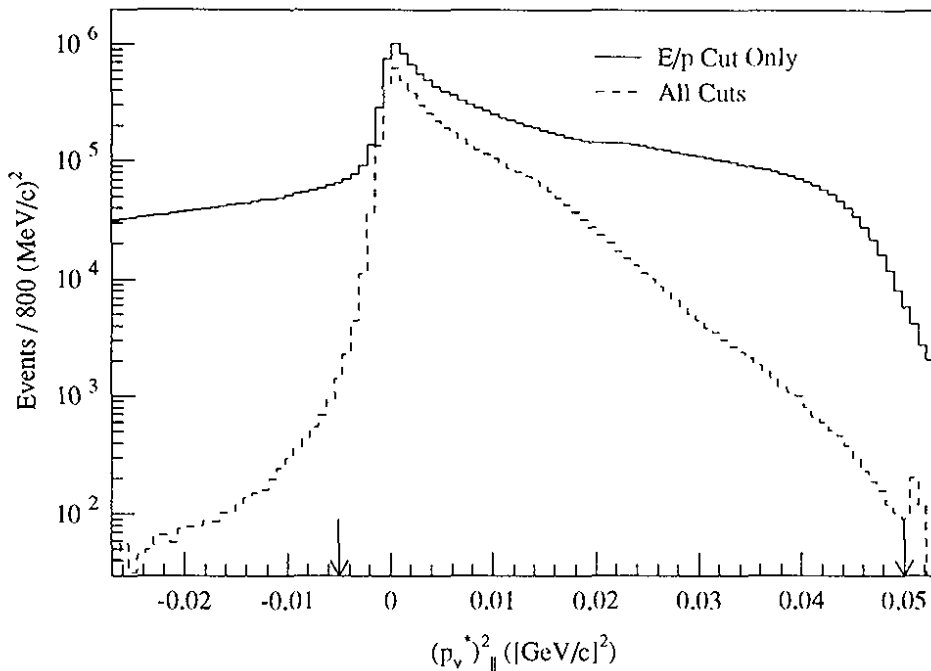
Figure 35. The Ke3 kinematic variable p_{\nu}^{*2} for Ke3 candidate calibration events after a loose E/p cut only (solid histogram), and after all but the kinematic cut (dashed histogram). The arrows indicate the analysis cut locations.
