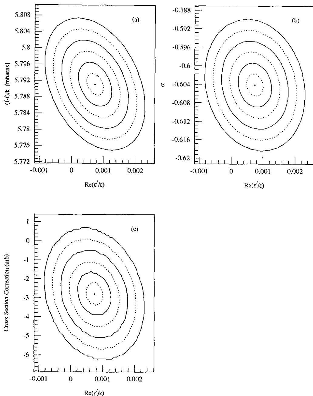
Figure 121. Contours of equal \chi^2 in the fit for \text{Re}(\epsilon'/\epsilon) . The contours are plotted in steps of 1/2 standard deviations. (a) [f(0) - \bar{f}(0)]/k|_{70\text{GeV}/c} versus \text{Re}(\epsilon'/\epsilon) . (b) \alpha versus \text{Re}(\epsilon'/\epsilon) . (c) Kaon-Carbon total cross section correction parameter (at 156 GeV/c) versus \text{Re}(\epsilon'/\epsilon) .
