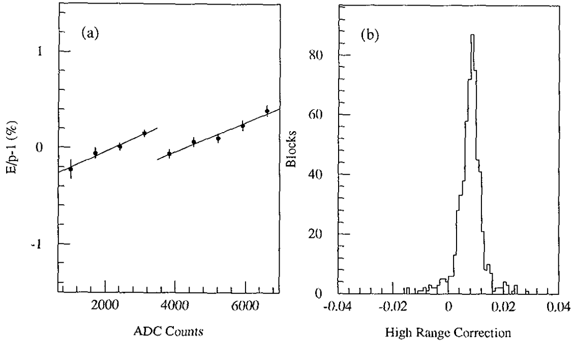
Figure 38. (a) E/p versus ADC counts for an individual block. The effect of the high range gain mismatch relative to the low range gain, coupled with the nonlinearity fit, clearly stands out. The gain mismatched by 0.6% of itself. (b) The fractional high range gain corrections for each corrected block.
