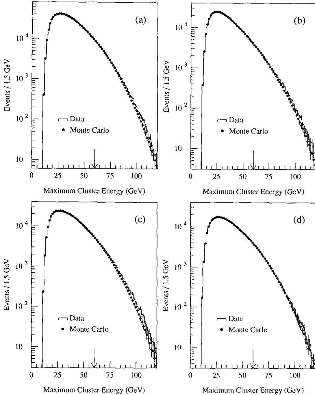
Figure 94. Distribution of the maximum cluster energy for 2\pi^0 decays in the data and the Monte Carlo simulation. The arrow indicates the position of the analysis cut. (a) Vacuum beam distributions for the entire data set. (b) Regenerator beam distributions for the entire data set. The regenerator beam distributions are plotted separately for (c) the 2\pi^0 subset with the lead sheet, and (d) the subset without the lead sheet. The background contributions have been included in all of the Monte Carlo overlays.
