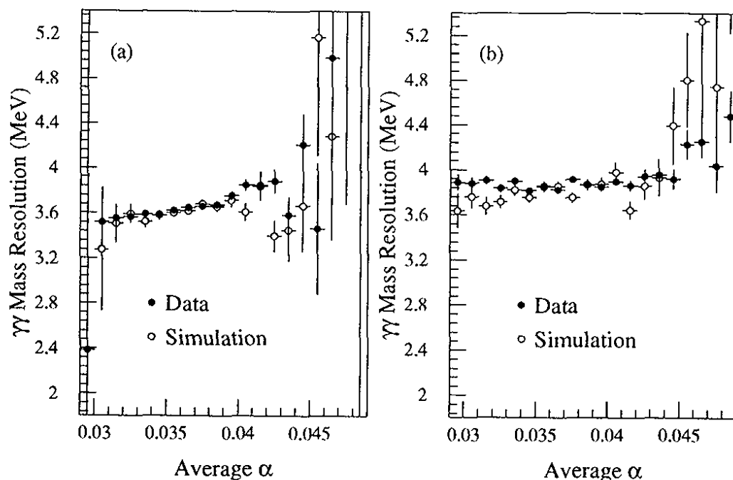
Figure 91. Resolution on the \gamma\gamma mass in \pi^+\pi^-\pi^0 data and Monte Carlo simulation. The resolution is plotted as a function of the average absorption coefficient \bar{\alpha} = (\alpha_1 + \alpha_2)/2 of the two photon clusters. (a) NC subset. (b) C2 subset.
