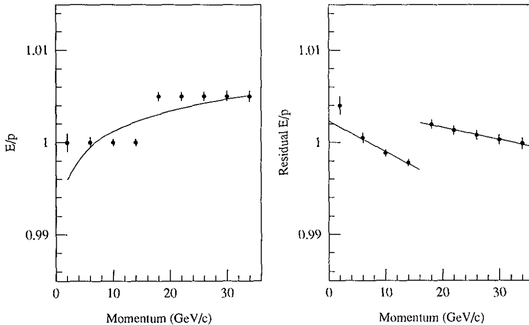
Figure 37. The distortion introduced into E/p by a 0.5% gain mismatch between the high and low ADC ranges. Left: E/p versus p with a gain mismatch, and the best fit nonlinearity which tries to compensate. The errors are representative of those available for an individual block. Right: The difference between the distorted E/p and the best fit nonlinearity. The linear fits in the high and low range regions yield a 0.51\% \pm 0.07\% measurement of the mismatch.
