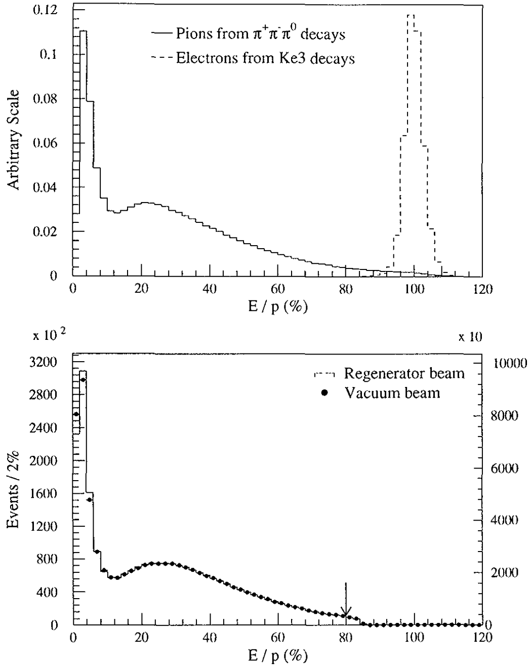
Figure 43. Shape of the E/p distribution for pions and electrons. (a) The solid histogram shows the spectrum for pions for a subset \pi^+\pi^-\pi^0 decays, and the dashed histogram shows the spectrum for electrons for a subset of \text{Ke3} decays. The normalization of the two samples is arbitrary. (b) The E/p distribution for pions from \pi^+\pi^- decays after all other cuts. The histogram shows the distribution for decays in the regenerator beam (left scale), and the dots show the distribution for decays in the vacuum beam (right scale). The cutoff at 0.85 is a result of the initial loose cut in the initial data reduction analysis pass. The final cut at 0.80 is indicated by the arrow.
