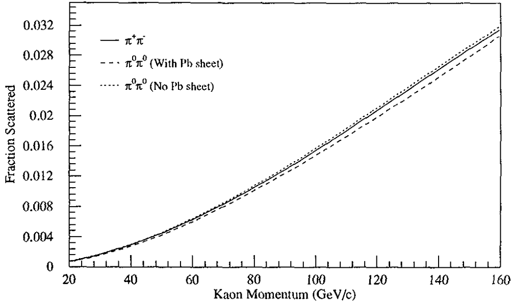
Figure 112. Fraction of kaons incident on the regenerator which have scattered in the shadow absorber. The fraction depends weakly on the relative beam and collimator positions, leading to the small differences in the different sets.
