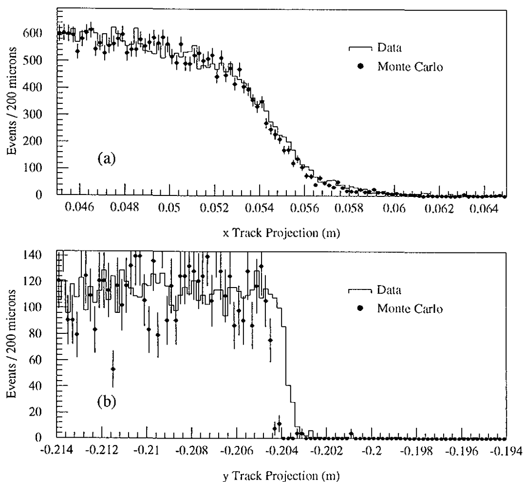
Figure 77. Illumination of two of the aperture edges by electrons from \text{Ke3} decays in the NC subset. The histogram shows the data illumination, while the dots show the MC prediction before the final tuning of the aperture positions. (a) Horizontal edge of the active mask. (b) East half of the bottom edge of the Collar Anti surrounding the lower beam. These edges showed the largest misalignment of their respective apertures before the final position adjustment. The mask edge is shifted about 230 microns, and the Collar Anti edge by about 700 microns.
