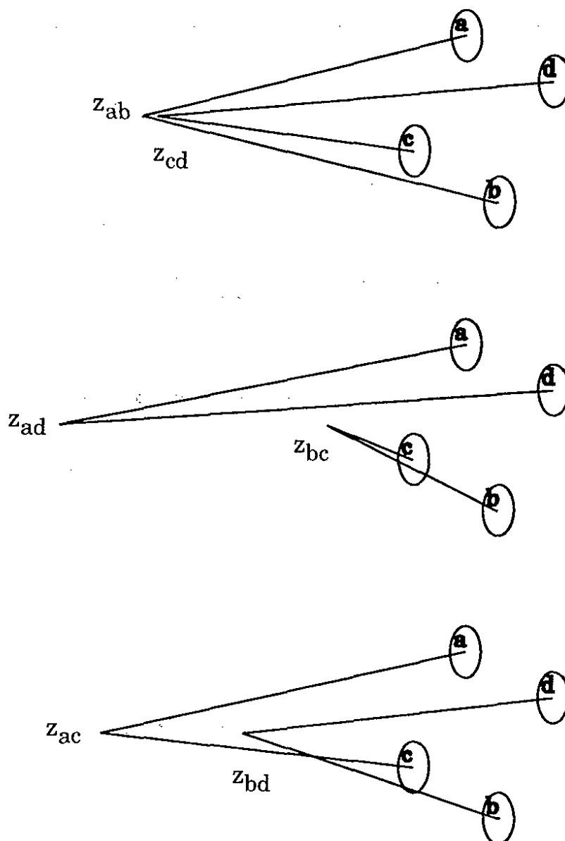
Figure 53. The z locations obtained for both \pi^0 decays in each of the three possible pairings of the four photons from a K \rightarrow \pi^0 \pi^0 decay. The top pairing will give the best \chi^2 for z_{ab} = z_{cd} .
