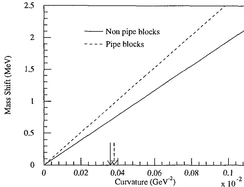
Figure 137. Mass shift as a function of the curvature of the quadratic cluster energy bias. The observed shift is shown for events with (dotted line) and without (solid line) clusters in the pipe blocks. The arrows indicate the average of the curvatures used in the systematic studies.
