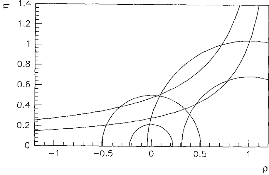
Figure 4. The one standard deviation constraints on \rho and \eta which result from the measurements of |\epsilon| , x_d and |V_{ub}|/|V_{cb}| . Plot courtesy J.R. Patterson.
