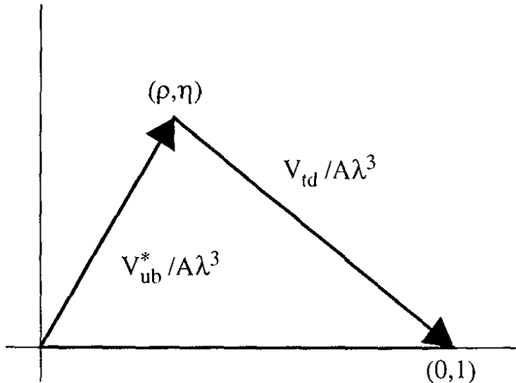
Figure 2. The unitarity triangle.
