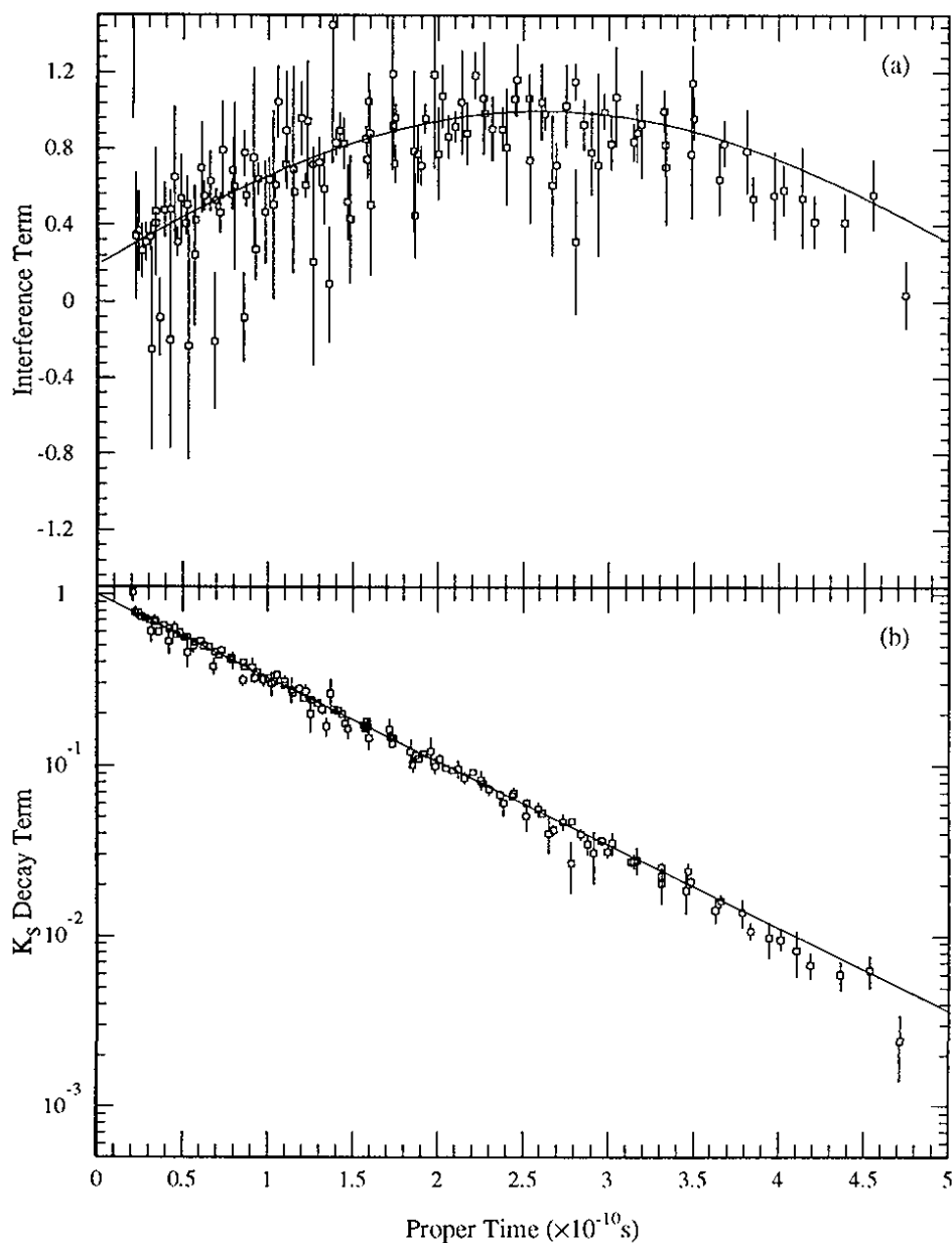
Figure 128. The interference and K_S decay curves measured for 2\pi^0 decays with momentum above 90 \text{ GeV}/c . (a) The average interference versus the average proper time in 1 \text{ m} by 10 \text{ GeV} bins. (b) The K_S decay term versus proper time, both measured at the center of the 1 \text{ m} by 10 \text{ GeV} bin. The \Delta m and \tau_S results from the grand fit to the 2\pi^0 data are shown as the curves.
