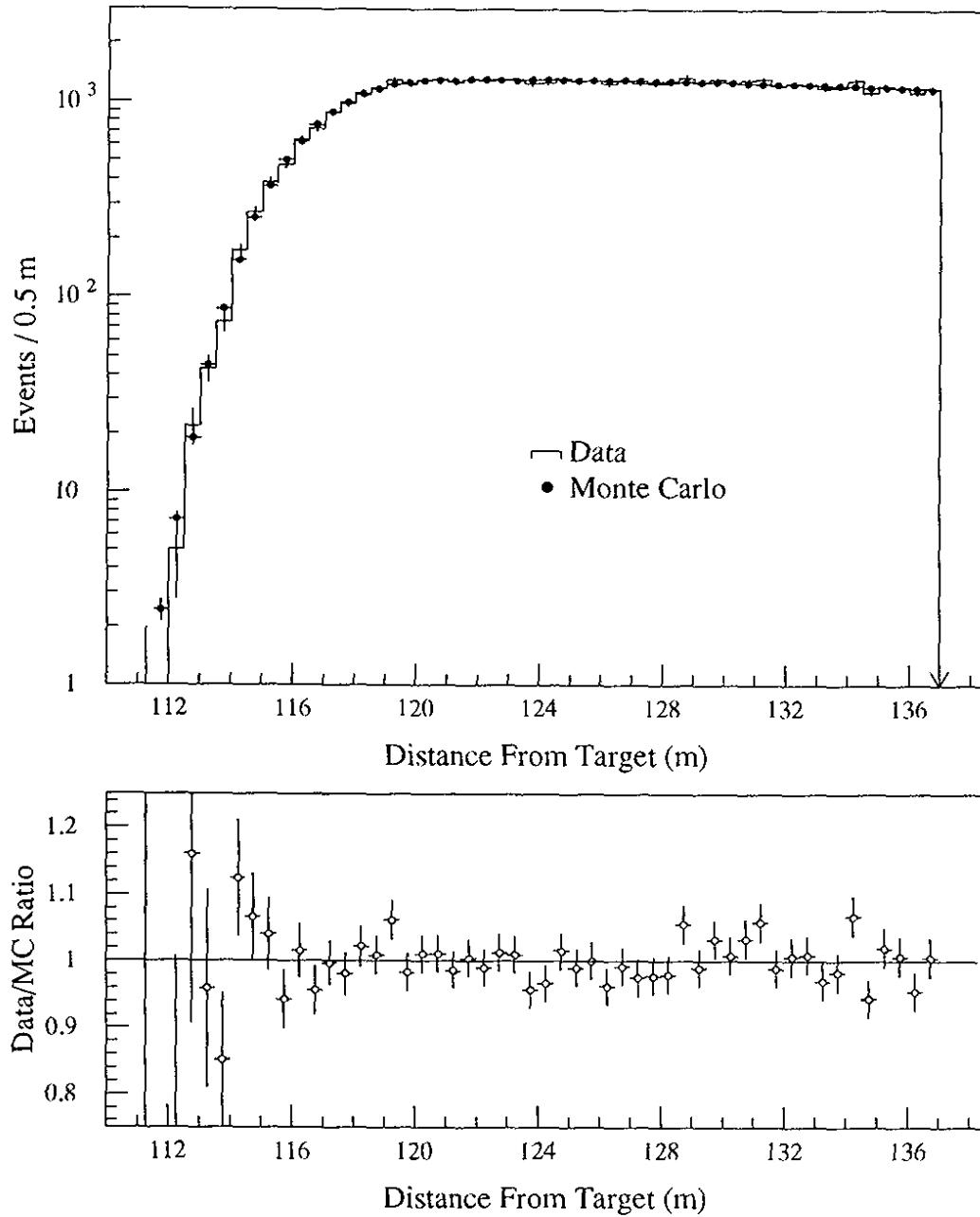
Figure 98. Vacuum beam z distribution for the \pi^+\pi^- data and Monte Carlo simulation in the 60 GeV/c to 70 GeV/c bin momentum bin. All final cuts have been made. Top : The z distribution for the two event samples, with the simulation statistics normalized to the data statistics. Bottom : The ratio of data events to simulated events in each 1/2 m bin.
