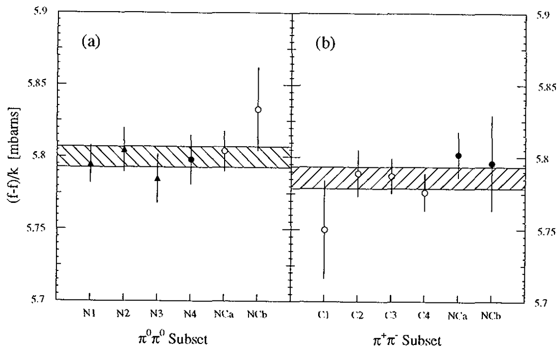
Figure 135. The regeneration amplitude measured in individual data subsets. The 2\pi^0 measurements are plotted in part (a) and the \pi^+\pi^- measurements in part (b). The one standard deviation bands from the fits to the entire 2\pi^0 or \pi^+\pi^- sample described in Section 9.1 have been plotted as well. The highest (lowest) intensity data for each mode is plotted with solid (hollow) points. In part (a), the subsets with (without) the lead sheet are indicated by triangles (circles).
