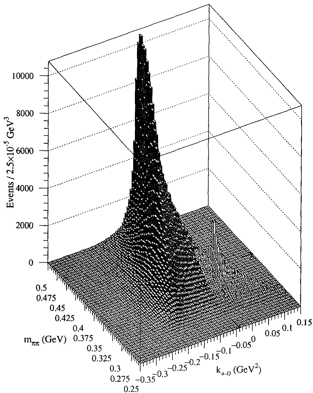
Figure 34. m_{\pi\pi} versus k_{+-0} in the Ke3 sample. The small peak at the lower right is due to \pi^+\pi^-\pi^0 background. Events in the lightly shaded region demarcated by the two arrows are removed from the final Ke3 sample.
