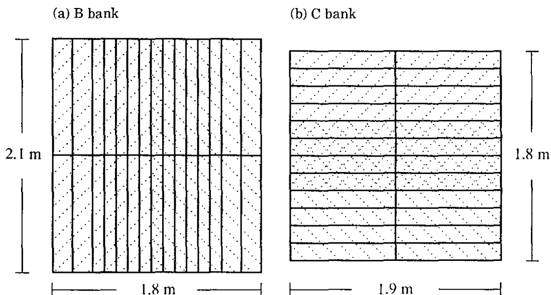
Figure 16. The B and C hodoscope banks used for charged triggering. The hatching illustrates the definition of the left and right "halves" in the B bank (and top and bottom "halves" in the C bank) used by the charged mode trigger. Staves with both directions of hatching are overlap regions which can belong to either half.
