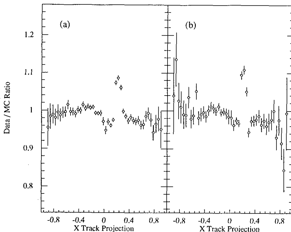
Figure 133. Ratio of the data and Monte Carlo track illumination at the lead glass when a 10% inefficiency is introduced into the response of two of the B hodoscope counters in the Monte Carlo. The two counters form a vertical stripe in the hodoscope bank. The data and Monte Carlo simulation are from the \pi^+\pi^- subset C4. (a) Regenerator beam ratio. (b) Vacuum beam ratio.
