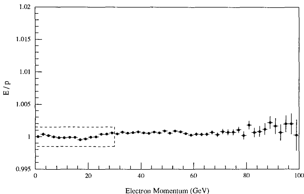
Figure 39. Mean value of the ratio of cluster energy to track momentum ( E/p ) versus momentum for electrons and positrons from Ke3 decays using the Ke3 calibration gains. The dashed box shows the momentum range used for the calibration.
