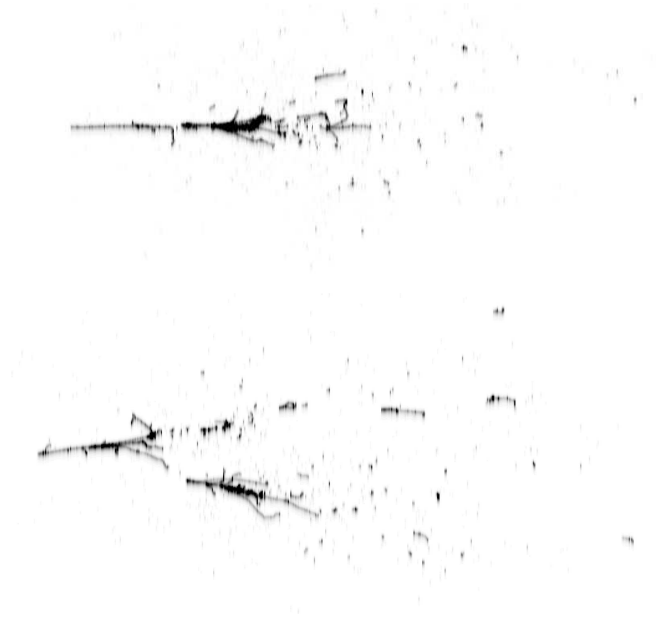
Fig. 1. Electromagnetic showers in the Liquid Argon TPC initiated by electron (upper part) and \pi^0 (lower part).
