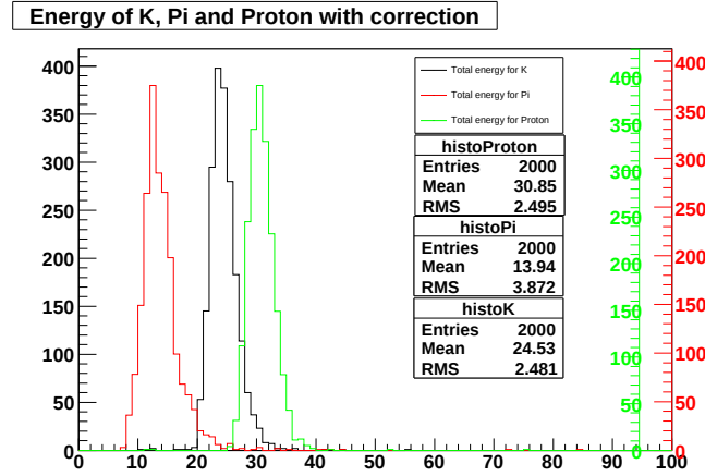
Fig. 3. Energy distribution for the total energy loss in 9 wires for the three particles ( \pi^+ , K^+ , p ) using the corrected energy loss.
