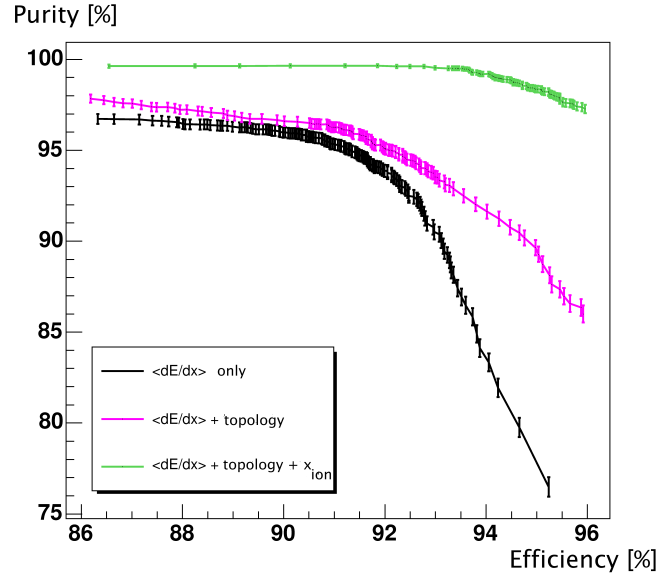
Fig. 2. Purity-efficiency plots for three levels of the analysis.
