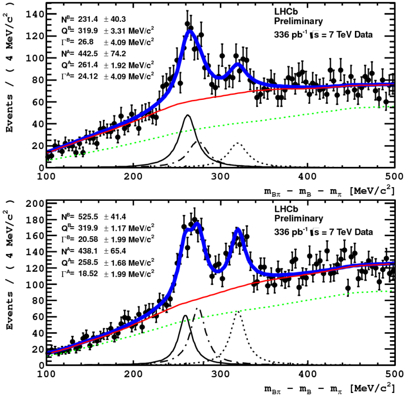
Fig. 5. The fit to the Q distributions of B\pi system. In both data plots the total fit functions are shown as thick black (blue) lines. The different components are shown as: light grey (green) for combinatorial background; dark grey (red) for sum of combinatorial background and associated production; black solid B_1 \rightarrow B^*\pi ; black dot-dashed for B_2^* \rightarrow B^*\pi ; black dotted for B_2^* \rightarrow B\pi .
