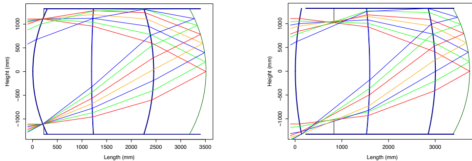
Figure 4. Baseline (left) and Advanced (right) designs.
