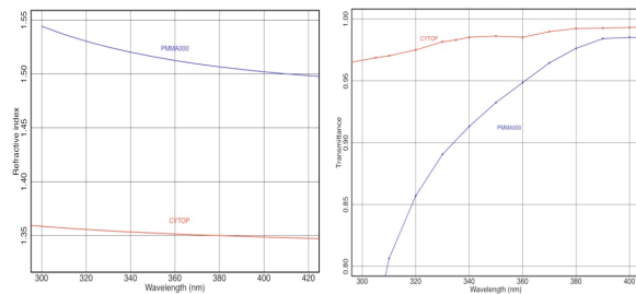
Figure 3. Left: refractive index for CYTOP and PMMA-000. Right: transmittance for CYTOP and PMMA-000 for 15-mm thickness.
