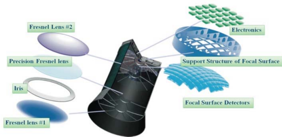
Figure 2. The main components of JEM-EUSO telescope concept.
