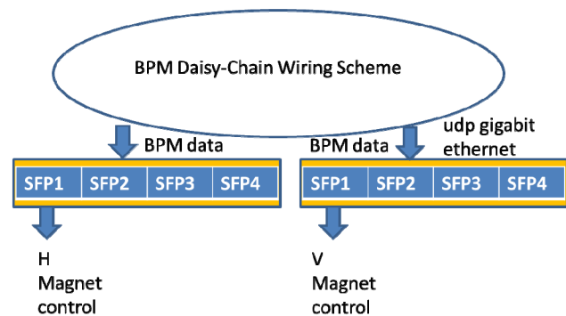
Figure 2: Feedback system is integrated by daisy-chain wiring bus of bpm with GDX module.
