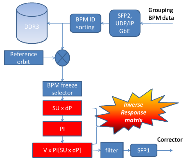
Figure 6: Control algorithm block diagram.
