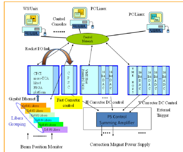
Figure 1: The overview system block diagram.
