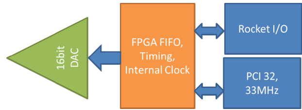
Figure 4: Functional block diagram of the corrector power supply control interface module. T. The fast setting from feedback engines will sum with slow setting from ILC.
