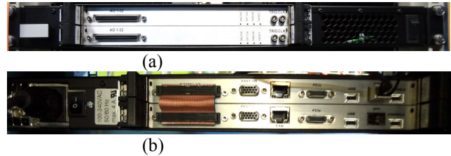
Figure 5:(a) CPSCI AO32 frontend. (b)CPSCI AO32 backend. 32 channels AO is extend to 64 channels AO by RTM-AO16 bus.
