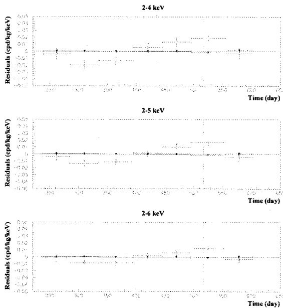
Figure 2: Experimental residual rates over the four DAMA/LIBRA annual cycles for single-hit events (open circles) (class of events to which DM events belong) and for multiple-hits events (filled triangles) (class of events to which DM events do not belong), in the energy intervals (2 – 4), (2 – 5) and (2 – 6) keV, respectively. They have been obtained by considering for each class of events the data as collected in a single annual cycle and by using in both cases the same identical hardware and the same identical software procedures. The initial time of the scale is taken on August 7 th . The experimental points present the errors as vertical bars and the associated time bin width as horizontal bars. See ref. 18 . Analogous results were obtained for the DAMA/NaI data in ref. 5 .
