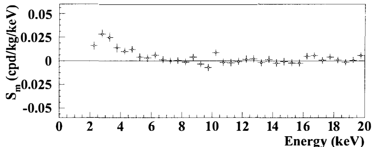
Figure 3: Energy distribution of the S_{m,k} variable for the total exposure of DAMA/NaI and DAMA/LIBRA: 0.82 ton \times yr. A clear modulation is present in the lowest energy region, while S_{m,k} values compatible with zero are present just above. In fact, the S_{m,k} values in the (6-20) keV energy interval have random fluctuations around zero with \chi^2/d.o.f. equal to 24.4/28. See ref. 18 .
