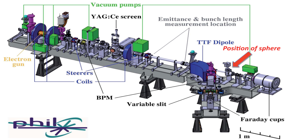
Figure 2: The PHIL accelerator: Futur position of the sphere is indicated with the red arrow
