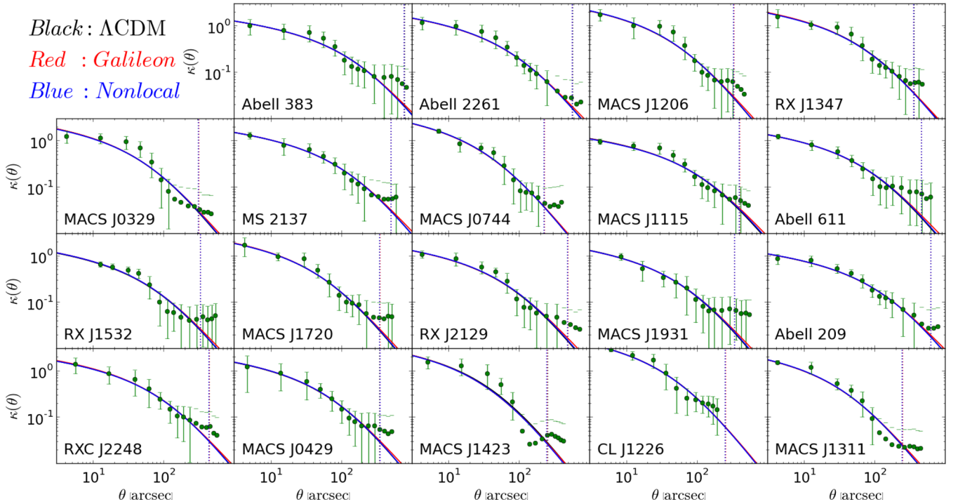
Figure 7. Best-fitting lensing convergence profiles, \kappa(\theta) = \Upsilon \kappa_\infty , obtained for all of the CLASH clusters assuming \Lambda CDM (black), Galileon gravity (red) and Nonlocal gravity (blue). The green dots are the radially binned data as described in Merten et al. (2015) and the error bars are the square root of the diagonal entries of the covariance matrix of the data. To guide the eye, the dotted vertical lines indicate the inferred values of R_{200} , which are barely distinguishable for the three models.
