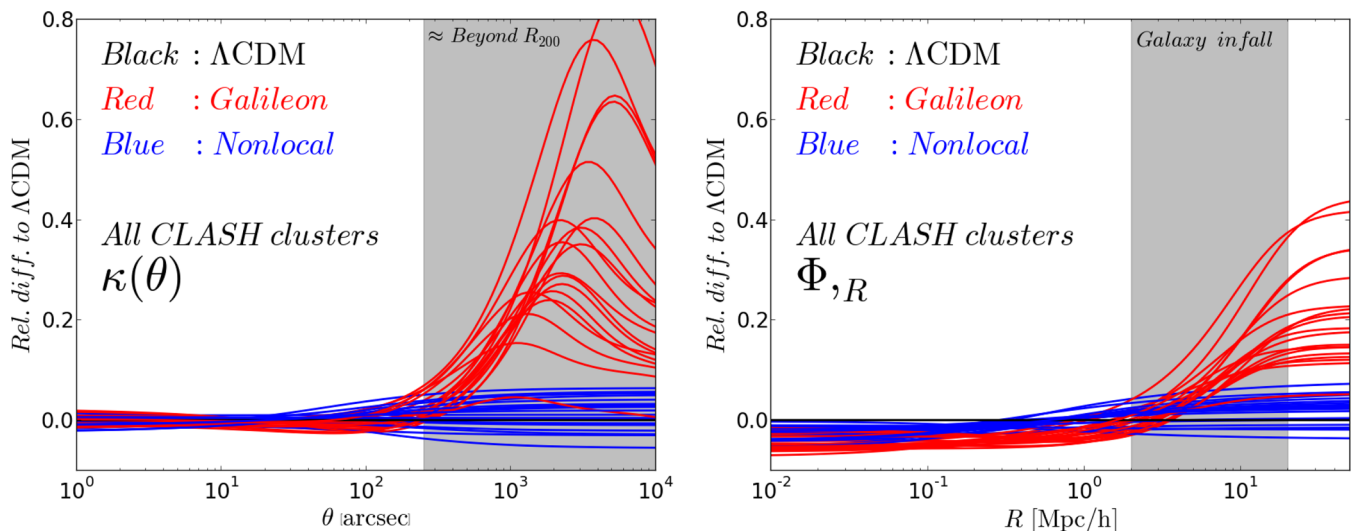
Figure 9. Left: best-fitting lensing convergence profiles, \kappa(\theta) = \Upsilon \kappa_{\infty} , for all of the CLASH clusters in the Galileon (red) and Nonlocal (blue) gravity models, plotted as the difference relative to the best-fitting profiles in \Lambda CDM (black). To guide the eye, the shaded band represents approximately the regions that lie beyond R_{200} for all clusters. Right: same as the left-hand panel, but for the total force profile \Phi_{,R} . The shaded band encloses the scales 2 \lesssim R \lesssim 20 \text{ Mpc } h^{-1} which are approximately those associated with the infall of surrounding galaxies.
