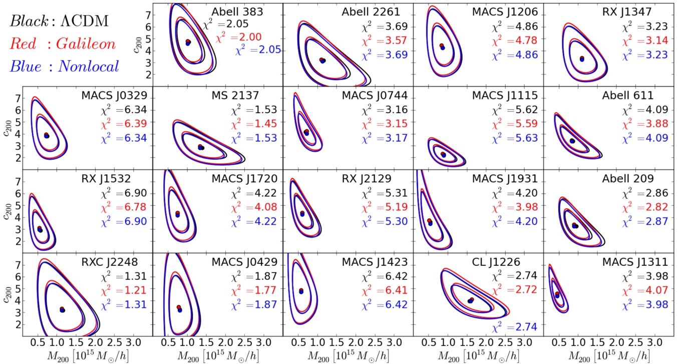
Figure 6. Two-dimensional 68 and 95 percent confidence limits on the c_{200} – M_{200} plane for all of the CLASH clusters assuming \Lambda CDM (black), Galileon gravity (red) and Nonlocal gravity (blue). The position of the best-fitting points is marked by the dots, and their respective \chi^2 values are shown in each panel.
