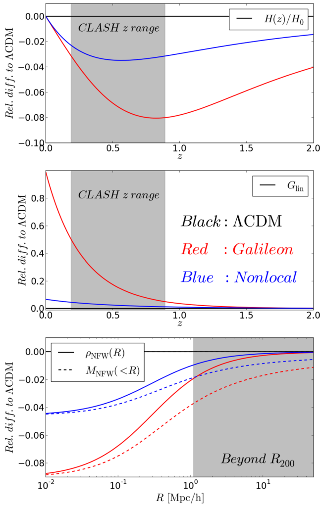
Figure 1. The upper and middle panels show, respectively, the time evolution of the Hubble expansion rate, H(z)/H_0 , and of the effective linear gravitational strength, G_{\text{lin}} , for the Galileon (red) and Nonlocal (blue) models, plotted as the relative difference to \Lambda CDM. The shaded band in these two panels indicates the redshift range spanned by the CLASH clusters analysed in this paper. The lower panel shows the density (solid) and enclosed mass (dashed) profiles for the Galileon (red) and Nonlocal (blue) models, plotted as the relative difference to \Lambda CDM. The NFW parameters and redshift are M_{200} = 5.0 \times 10^{14} M_\odot h^{-1} , c_{200} = 4.0 , z_d = 0.5 . To guide the eye, the shaded band in the lower panel indicates the radial scales outside R_{200} in \Lambda CDM.
