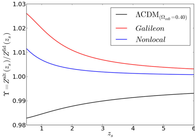
Figure 3. Dependence of the factor \Upsilon = Z^{\text{alt}}(z_s)/Z^{\text{fid}}(z_s) , equation (52), on the source redshift z_s for a \Lambda\text{CDM} model with \Omega_{m0} = 0.4 (black), Galileon gravity (red) and Nonlocal gravity (blue). The cosmological background of these models is different from the fiducial \Lambda\text{CDM} model with \Omega_{m0} = 0.27 used by Merten et al. (2015). In this figure, z_d = 0.35 , which is typical for the CLASH clusters.
